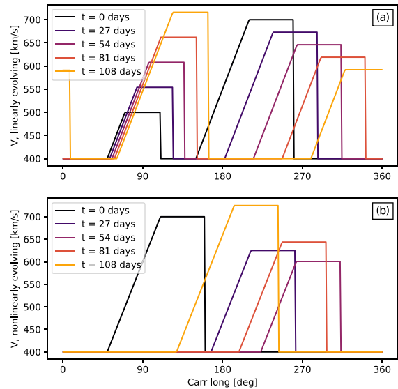
Figure 1. Two models of solar-wind speed evolution. Snapshots of solar-wind speed as a function of Carrington longitude are shown five times, approximately one Carrington rotation (CR) apart. Panel (a): Two fast solar-wind streams evolve linearly in magnitude, width, and position as a function of time. Panel (b): A single solar-wind stream evolves non-linearly in magnitude, width, and position as a function of time.
