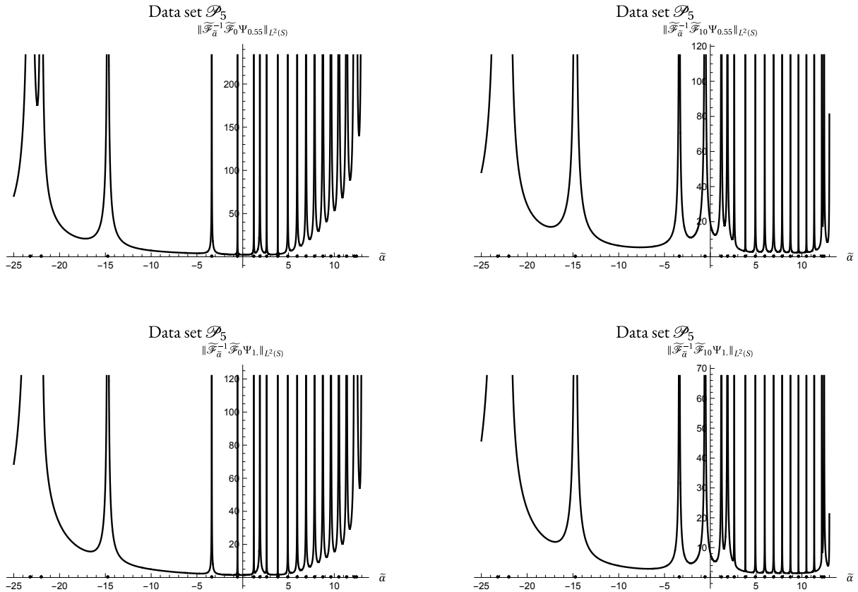
Figure SM1: Plots of the norms of f_{A,t} for different choices of A and t for dataset \mathcal{P}_5 .
