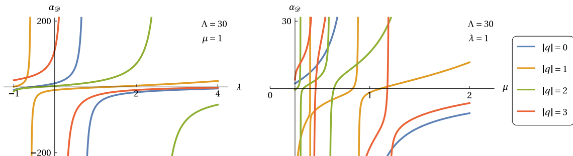
Figure 3: Some eigenvalues \alpha_{\mathcal{D}_\Lambda} of the nnDtN map for a unit disk as functions of \lambda (left figure) and \mu (right figure) for fixed \Lambda = 30 .
