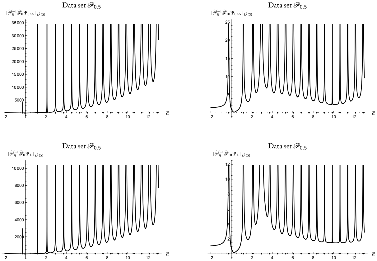
Figure SM2: Plots of the norms of f_{A,t} for different choices of A and t for dataset \mathcal{P}_{0.5} .
