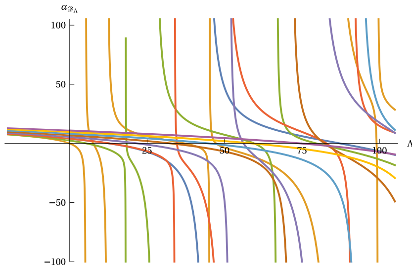
Figure 1: Some eigenvalues \alpha_{\mathcal{D}_\Lambda} of the nnDtN map for the unit disk as functions of \Lambda . Here \lambda = \mu = \rho_s = 1 .
