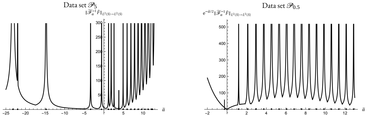
Figure 5: Plots of the operator norms \|\widetilde{\mathcal{F}}_{\tilde{\alpha}}^{-1} \widetilde{F}_{\tilde{\alpha}}\|_{L^2(S) \rightarrow L^2(S)} as functions of \tilde{\alpha} . Additional exponential scaling for data set \mathcal{P}_{0.5} improves the appearance.
