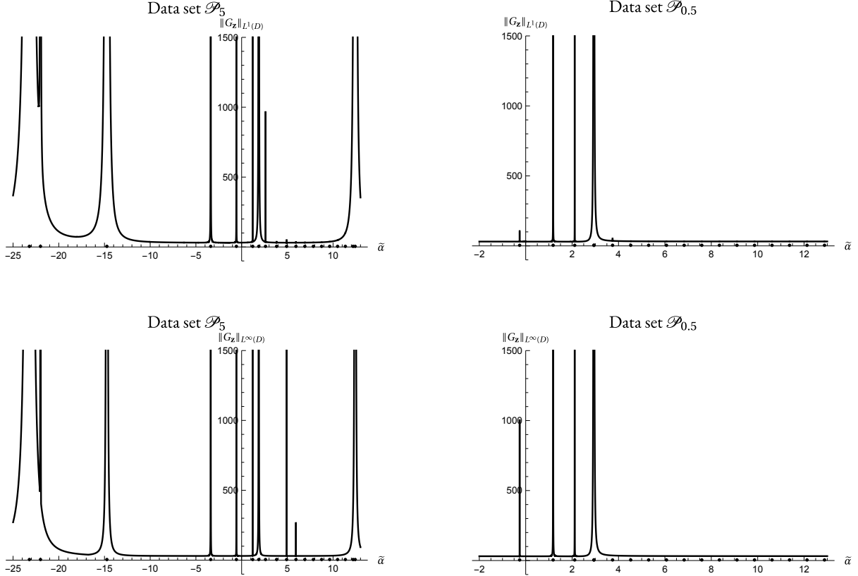
Figure 4: Plots of the norms \|G_z\|_{L^\infty(D)} and \|G_z\|_{L^1(D)} as functions of \tilde{\alpha} . In this and subsequent Figures, the black dots on the \tilde{\alpha} axis indicate the positions of the eigenvalues of \mathcal{D}_\Lambda from the corresponding column of Table SM1.
