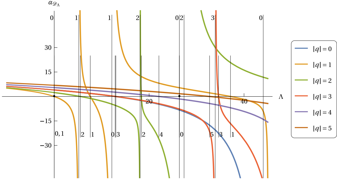
Figure 2: Zoom of Figure 1 that shows eigenvalues \alpha_{\mathcal{D}_\Lambda} with the angular momentum |q| \leq 5 , see §SM1 for details. The short vertical lines indicate the positions of the Neumann eigenvalues \Lambda_{\text{Neu}} (labelled with a corresponding angular momentum |q| ), where the curves \alpha_{\mathcal{D}_\Lambda} corresponding to the eigenmodes with the same angular momentum cross the line \Lambda = 0 . The long vertical lines indicate the positions of the mixed eigenvalues \Lambda_{\text{mix}} (labelled with a corresponding angular momentum |q| ), where the curves \alpha_{\mathcal{D}_\Lambda} corresponding to the eigenmodes with the same angular momentum blow up. All the curves and eigenvalues corresponding to |q| > 0 are in fact double. We note that \Lambda = 0 and \Lambda \approx 26.3746 , marked with black dots, are Jones eigenvalues for the disk with the angular momentum of the corresponding eigenmode being q = 0 ; therefore the corresponding curves \alpha_{\mathcal{D}_\Lambda} have neither a zero nor a singularity at these values of \Lambda , see Remark 2.5.
