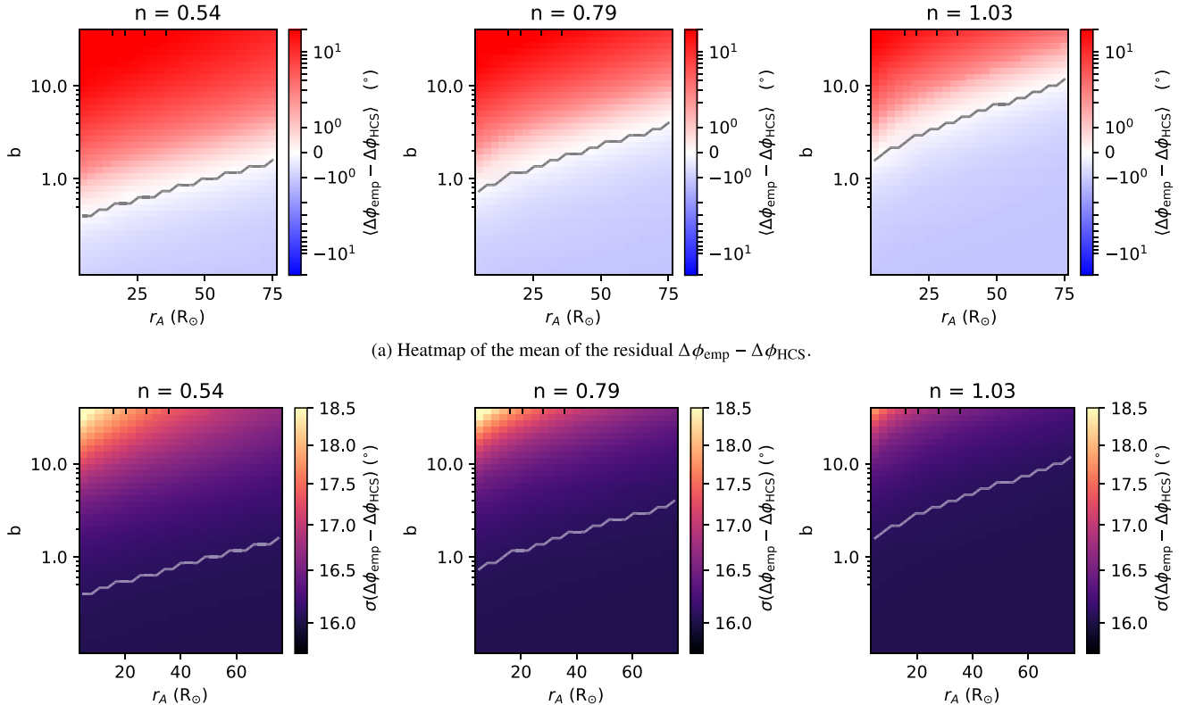
(b) Heatmap of the standard deviation of the residual \Delta\phi_{\text{emp}} - \Delta\phi_{\text{HCS}} . The line of minimum absolute mean residual from 6a is shown in white.
