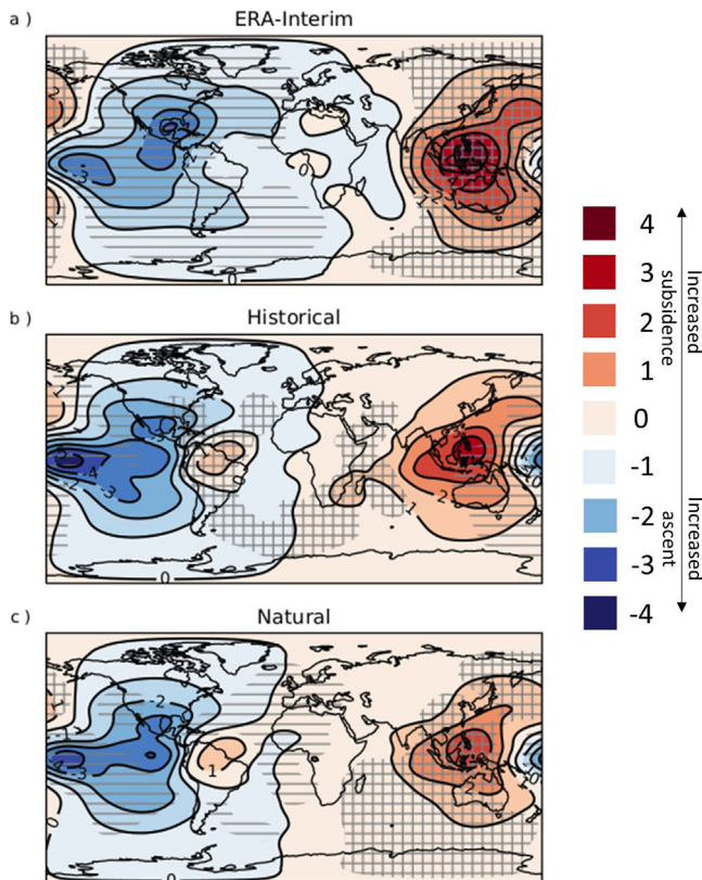
FIGURE 2 October–February velocity potential ( 10^6 \text{ m}^2/\text{s} ) composite difference between El Niño and La Niña years at 200 hPa for (a) ERA-Interim reanalysis; (b) historical ensemble; (c) natural ensemble. Hatching shows where El Niño composites are significantly different from La Niña years for (a), where historical is significantly different from Era-Interim for (b) and where natural is significantly different from historical for (c). Horizontal lines and cross-hatching indicate decreased and increased significance at the 10% level, respectively. Positive values (red colours) are associated with increased subsidence while negative values (blue colours) are associated with increased ascent
