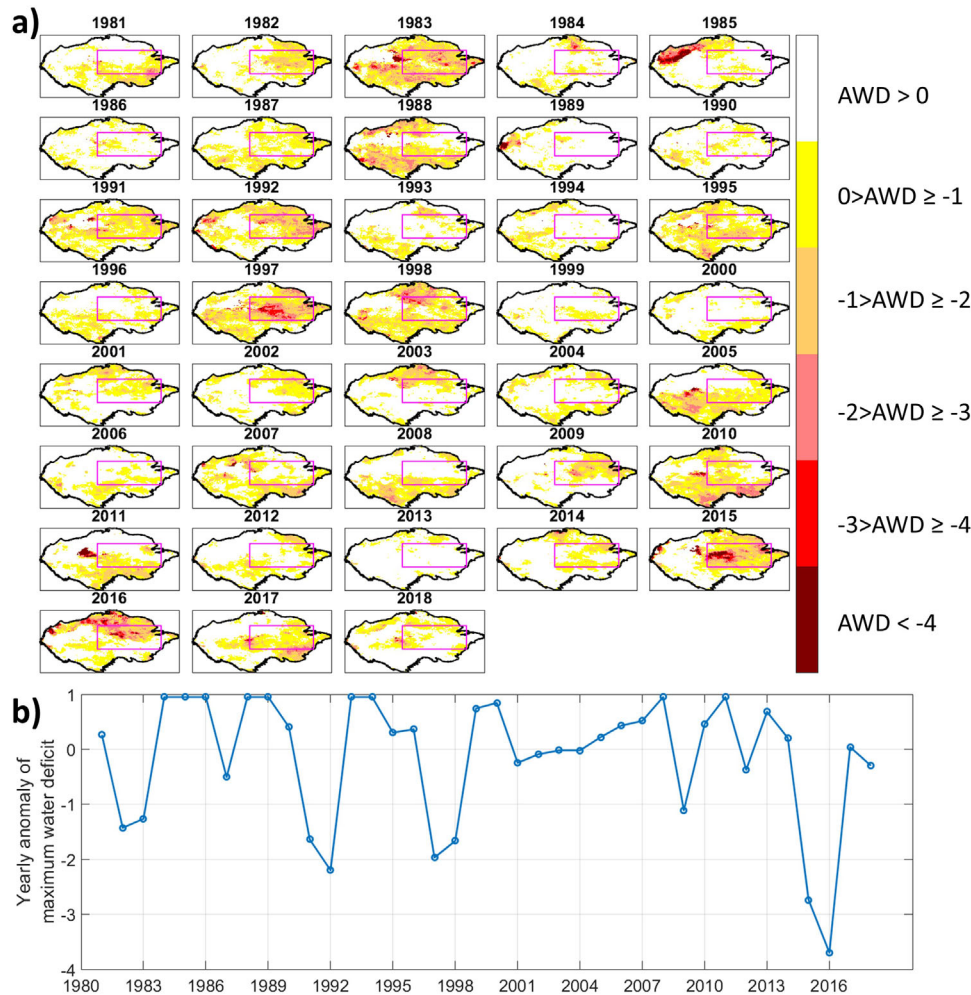
FIGURE 1 (a) Spatial variation of yearly anomaly of maximum water deficit (AWD) for the Amazon basin and location of the study area (purple rectangle 2^{\circ} N to 8^{\circ} S and 65^{\circ} W to 50^{\circ} W); (b) time series of AWD for the study area
