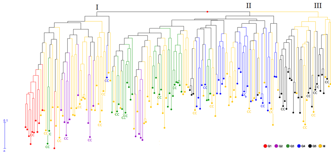
1 2 Fig. 2 Neighbor-joining dendrogram based on the Dice similarity index showing the relationships among 181 3 hazelnut genotypes from WHGC. Genotypes are colored according to their assignment to the different gene pools, 4 as inferred by STRUCTURE software at K = 5: Central Europe (Q1), British Islands (Q2), Iberian Peninsula (Q3), 5 Italian Peninsula (Q4), Balkans-Black Sea (Q5), and mosaic group (M). Entries of the final core collection (Cv- 6 Dce30) are reported as CC
