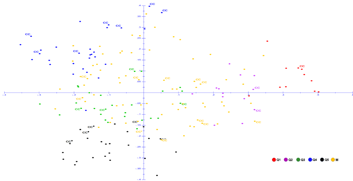
7 8 Fig. 3 Two-dimensional PCoA scatterplot of 181 hazelnut genotypes from WHGC based on Dice's distance. 9 Genotypes are colored according to their assignment to the different gene pools, as inferred by STRUCTURE 10 software at K = 5: Central Europe (Q1), British Islands (Q2), Iberian Peninsula (Q3), Italian Peninsula (Q4), 11 Balkans-Black Sea (Q5), and mosaic group (M). Entries of the final core collection (Cv-Dce30) are reported as 12 CC
