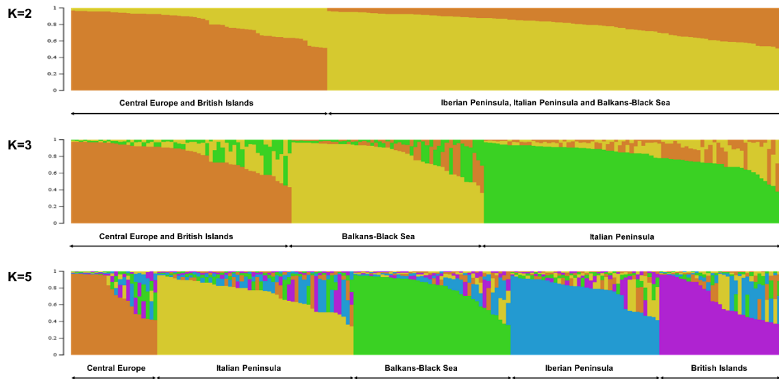
12 13 Fig. 1 Population structure and hierarchical organization of genetic relatedness of 181 genotypes from the whole 14 hazelnut germplasm collection (WHGC) at K = 2, K = 3, and K = 5, as inferred by STRUCTURE software 15
