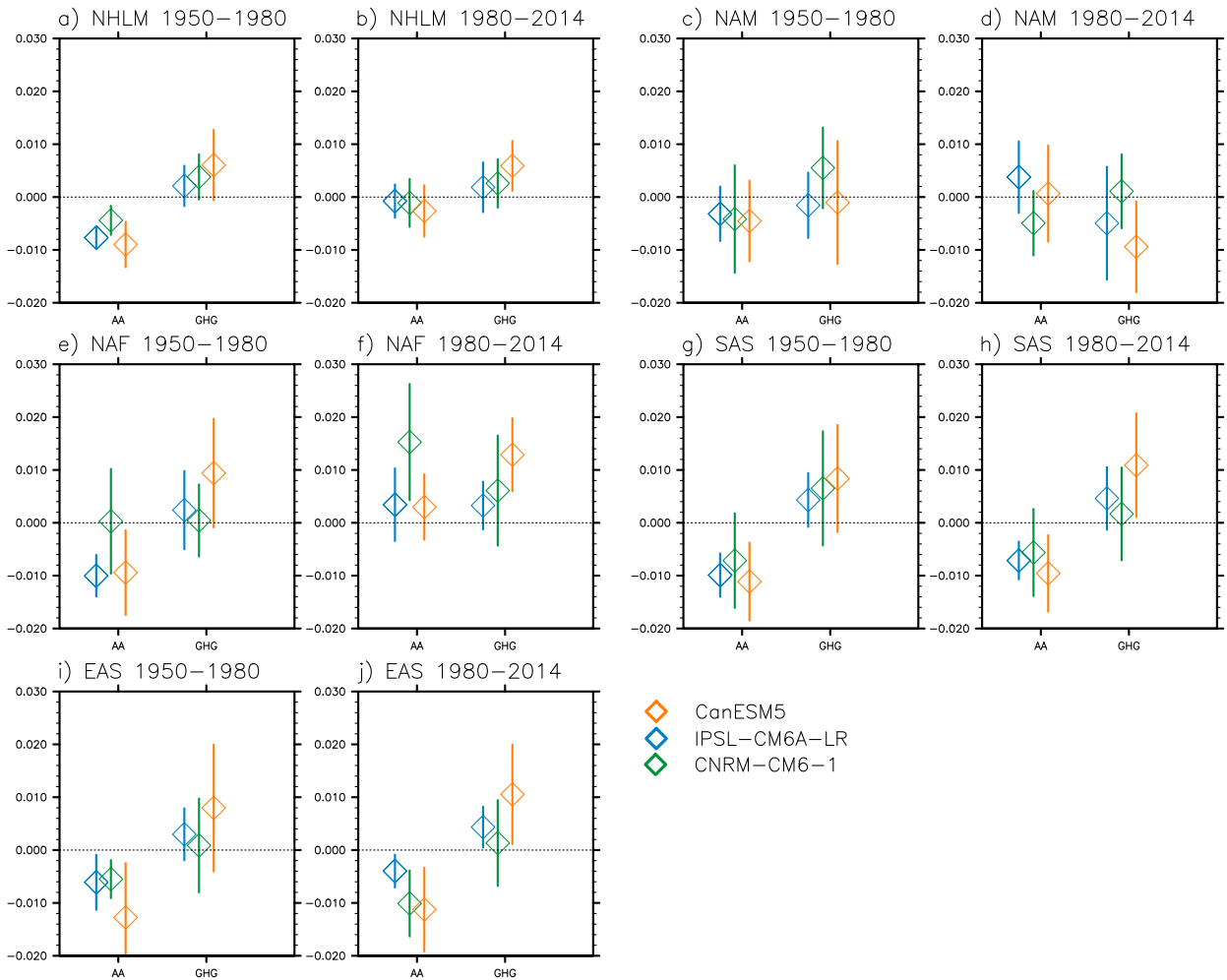
FIG. 11. Ensemble-mean in precipitation trends ( \text{mm day}^{-1} \text{yr}^{-1} ) in MJJAS for (a),(b) NHLM, (c),(d) NAM, (e),(f) NAF, (g),(h) SAS, and (i),(j) EAS monsoon domains, associated with the AA and GHG effects. Trends are computed over the periods (a),(c),(e),(g),(i) 1950–80 and (b),(d),(f),(h),(j) 1980–2014. The marker indicates the ensemble mean and the vertical lines the ensemble standard deviation. Results are given for three models: CNRM-CM6-1 (green; 10 members), IPSL-CM6A-LR (blue; 10 members), and CanESM5 (orange; 30 members).
