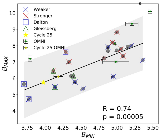
Figure 4. B_{Max} versus B_{Min} at the end of the previous cycle. The black line shows the correlation with a correlation coefficient of \sim 0.74 and a p-value of 0.00005. Gray shaded area represents uncertainty with 95% confidence level. Gray circles represent data points for each cycle, and blue (or red) x signs mark cycles that are predicted to be weaker (or stronger) than their previous cycles. Considering only the inconclusive cycles provides a better correlation ( R = 0.95 and p = 0.0009 ). Blue (or green) squares (or triangles) enclose cycles associated with the Dalton (or Gleissberg) period. Green circles with error bars represent datapoints from OMNI data set. The yellow star (circle with error bar) shows our prediction for SC25 based on SC24 B_{Min} from Rahmanifard (2017) (or OMNI data).
