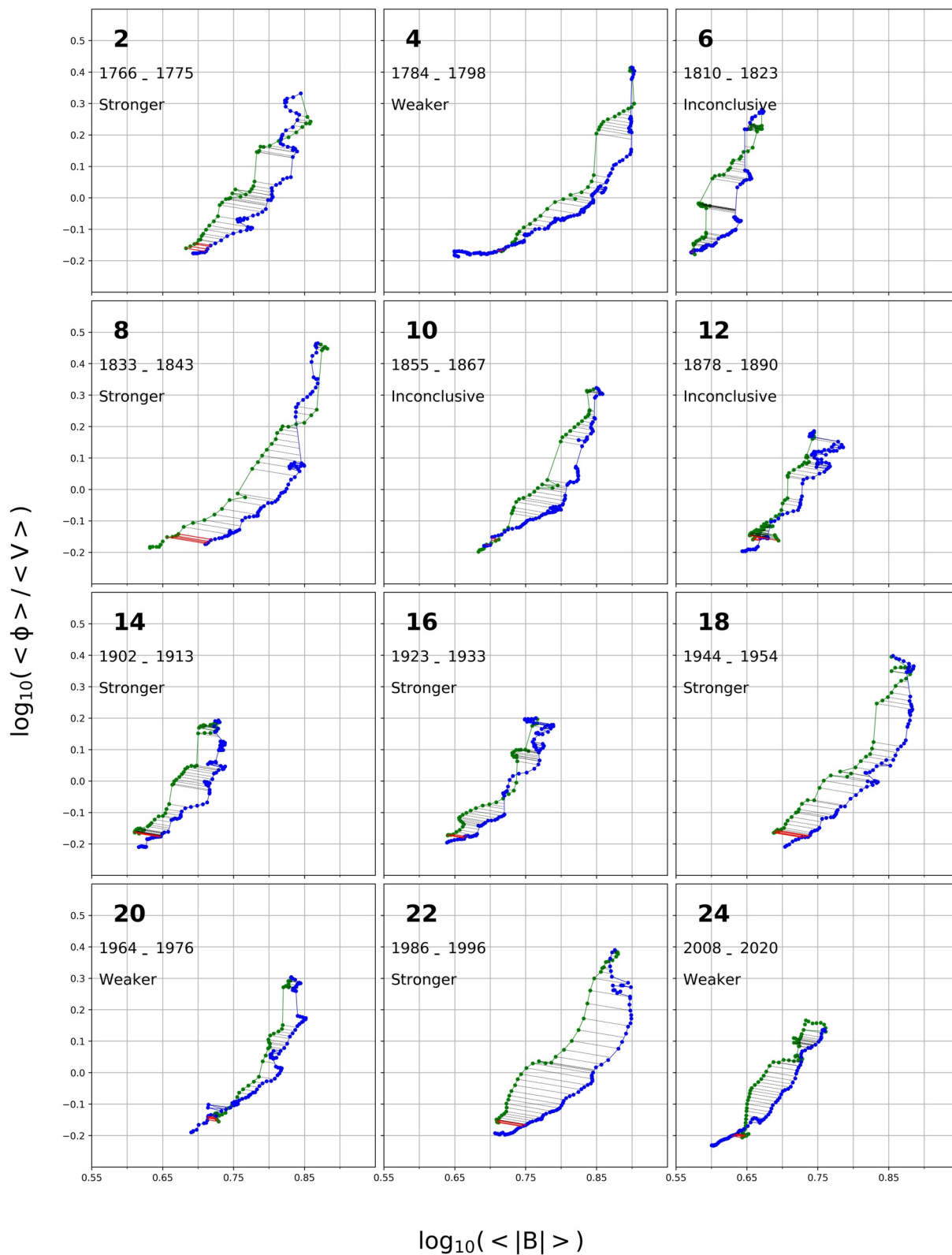
Figure 3. Correlation diagrams for even cycles. Green data points represent the first half of cycles, and blue data points denote the second half of cycles. Dashed black lines that connect the two halves are used to find the distance between the two halves. Red solid lines that connect the start of the two halves are used to determine if the cycle is open.
