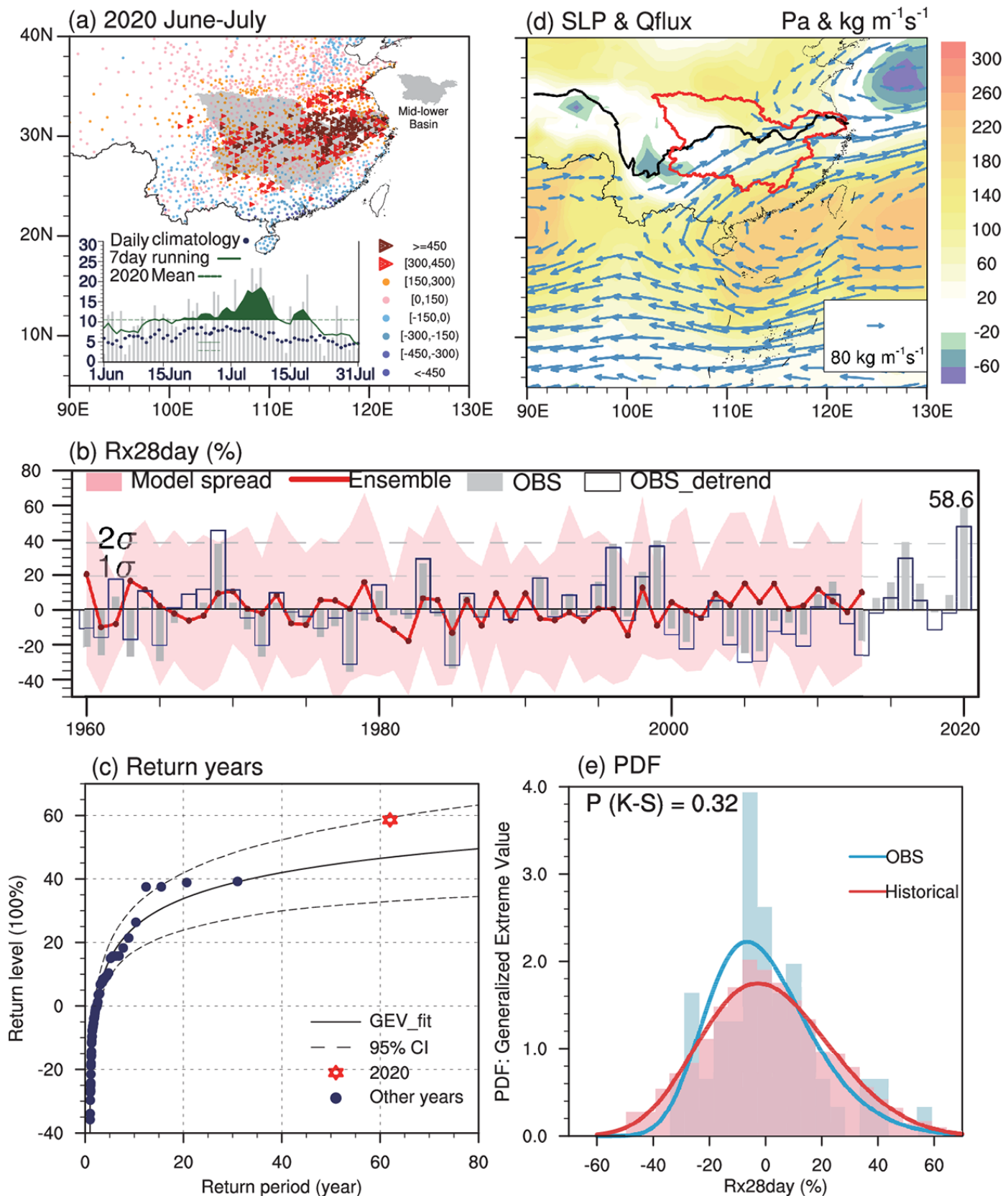
Fig. 1. (a) Observed accumulated precipitation (AP) anomalies (mm) during JJ 2020, with inset showing the daily rainfall evolution of which dashed green line for the mean value, green curve for 7-day running average, and blue dots for the daily climatology. (b) Time series of regional mean Rx28day% for observations (bar) and Historical simulations (red line and pink shading). (c) Return periods of observed Rx28day% in GEV fit with 90% uncertainty range, with a red star for the 2020 event and blue circles for other years. (d) Anomalies of SLP (shading; Pa) and column-integrated water vapor flux (vectors; \text{kg m}^{-1} \text{s}^{-1} ) during JJ 2020. The MLYRB is highlighted in red. (e) PDFs of Rx28day% for observations (blue) and Historical simulations (red) with p value for the K-S test.
