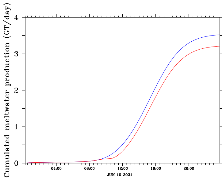
Figure 14. MAR-simulated whole Greenland Ice Sheet cumulative surface melt production (units Gt/day) integrated for 10 June 2021 with (red line) and without (blue line) the solar eclipse.
