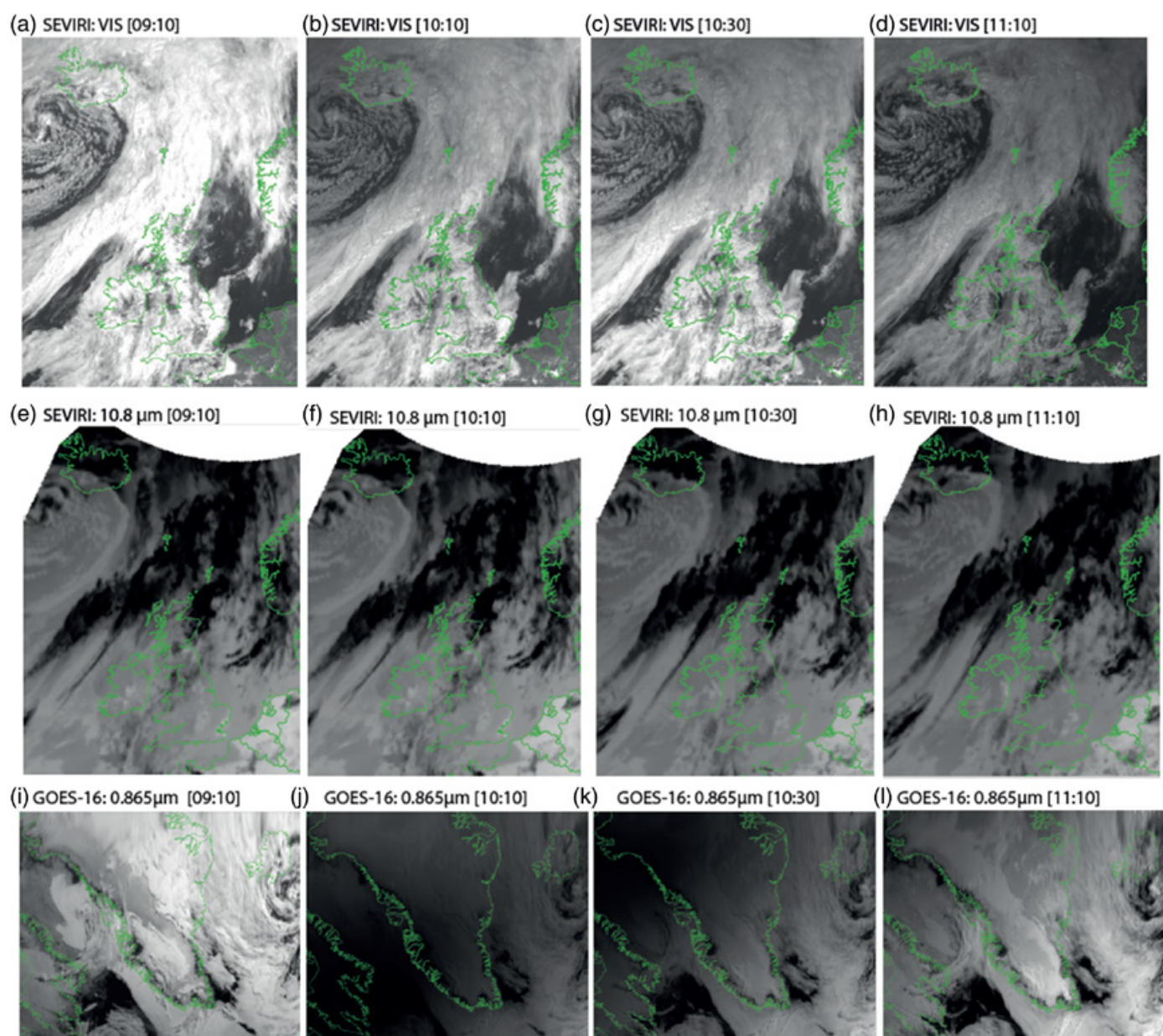
Figure 3. Satellite greyscale image sequences, showing cloud cover conditions during the eclipse period: (a–d) SEVIRI high-resolution visible broad bandwidth (0.6–0.9µm) images and (e–h) SEVIRI Ch9 thermal infrared, for the British Isles/Iceland; panels (i–l) show GOES 16 CM-03 (0.865µm) images of Greenland/Iceland. The eclipse shadow is evident in (j) and (k).
