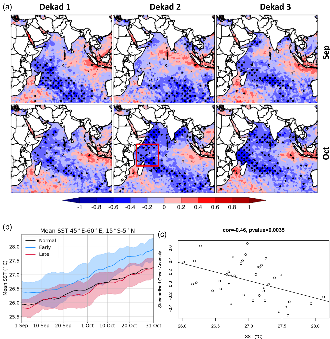
FIGURE 6 Correlation of the SST and the short rains onset anomaly from CHIRPS from 1981 to 2019. (a) Onset anomaly correlation and the SST for each grid point over the Indian Ocean Basin. The black dots represent correlations that are statistically significant at the 5% significance level. (b) Evolution of the SST over western Indian Ocean ( 45^{\circ} – 60^{\circ} E and 15^{\circ} S– 5^{\circ} N). The shading in the plot represents the standard deviations of the SST. (c) Relationship of SST and onset anomaly utilizing the box 45^{\circ} – 60^{\circ} E and 15^{\circ} S– 5^{\circ} N for the second dekad of October
