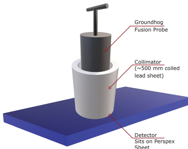
FIGURE 7 Scheme diagram showing the Groundhog ® detector in its collimated configuration. Source: Drawn by authors [Colour figure can be viewed at wileyonlinelibrary.com ]
