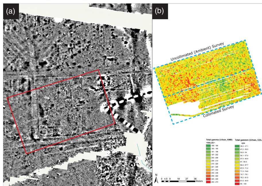
FIGURE 2 Comparison of fluxgate gradiometry data ( \pm 7nT ) (a) against total gamma radiation data (b) collected at the Urban Area (Site A). Both collimated and uncollimated radiation measurements are presented. Radiation data are displayed in cps. No clear anomalies have been identified. An area of increased activity in the bottom right corner of the survey area may be attributable to a modern feature (buried pipe). An area of elevated activity to the left of the survey area broadly aligns with the cross road. However, due to its distribution, it may be a naturally occurring feature. Source: Fluxgate gradiometry data source: Silchester Mapping Project Creighton and Fry (2016) plus own (primary) data [Colour figure can be viewed at wileyonlinelibrary.com ]
