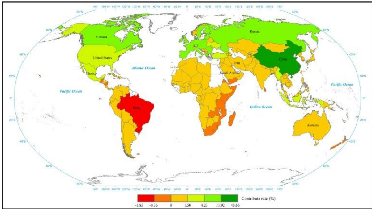
Fig. 7. The contribution rates (%) of each country in restoring global karst ecosystem productivity. The countries of the European Union (EU) are considered together given the large total karst area and relatively small size of some EU countries.
