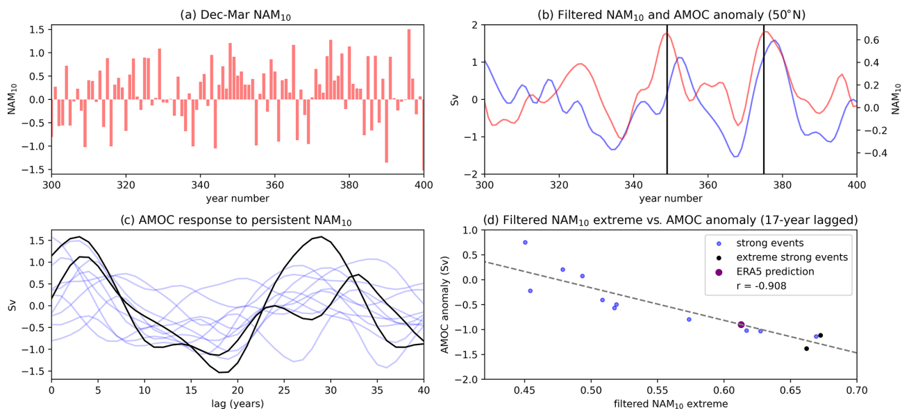
Figure 13. (a) Dec–Mar NAM_{10} index (red bars) from the UKESM simulation between year numbers 300 and 400. (b) AMOC (blue) and NAM_{10} (red) indices smoothed with the Gaussian filter ( \sigma = 2 years) between year numbers 300 and 400 of the UKESM simulation. Black vertical lines show the location of the largest smoothed NAM_{10} (c) AMOC response to persistent strong NAM_{10} intervals. Light blue lines denote lagged AMOC responses of the AMOC from the whole UKESM simulation, and black lines show AMOC responses to NAM_{10} intervals marked in (b) by vertical black lines. (d) Scatterplot of filtered NAM_{10} index values occurring at persistent strong NAM_{10} intervals throughout the whole UKESM simulation (y axis) against AMOC anomalies at 50^\circ N lagged 17 years after the persistent intervals' central year (x axis). Blue points indicate persistent intervals, and black dots represent the two intervals displayed in panel (b). The dotted line represents the linear line of the best fit for the points in black and blue. Also included is the 17-year lag AMOC anomaly predicted by projecting the regression coefficients used to construct the linear fit onto the maximum smoothed NAM_{10} index in the ERA5 dataset (purple point).
