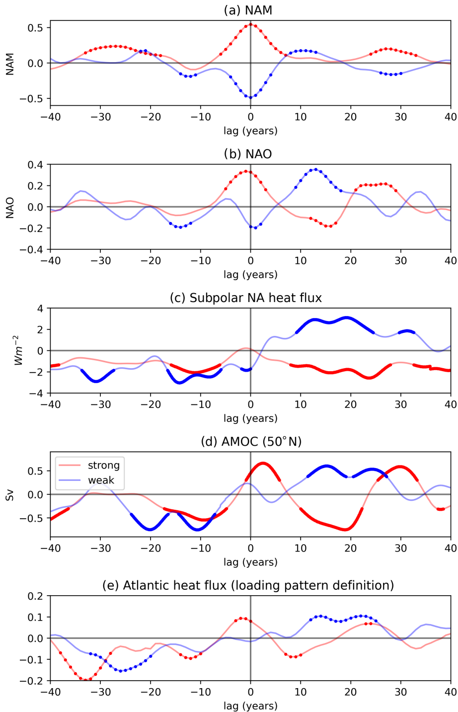
Figure 5. (a) Composites of (a) Gaussian smoothed NAM_{10} , (b) NAO, (c) subpolar NA heat flux, (d) AMOC anomalies at 50^\circ N, and (e) a NA heat flux index derived by projecting the Dec–Mar heat flux onto the response pattern in Fig. 6 that are associated with persistent vortex intervals of different types. On each subfigure, the red (blue) plots show the lead/lag responses to composites of strong (weak) persistent NAM_{10} intervals. Solid dots denote composite anomalies are significant to the 95 % level under a two-tailed Student’s t test.
