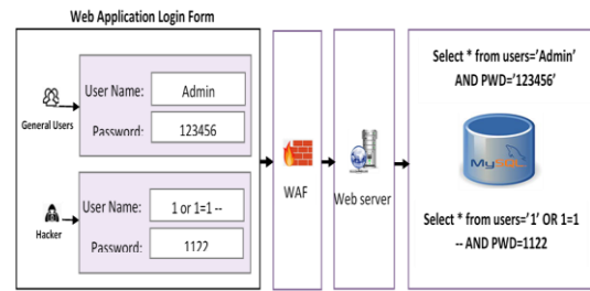
Fig. 1. SQL Injection Attack Process
