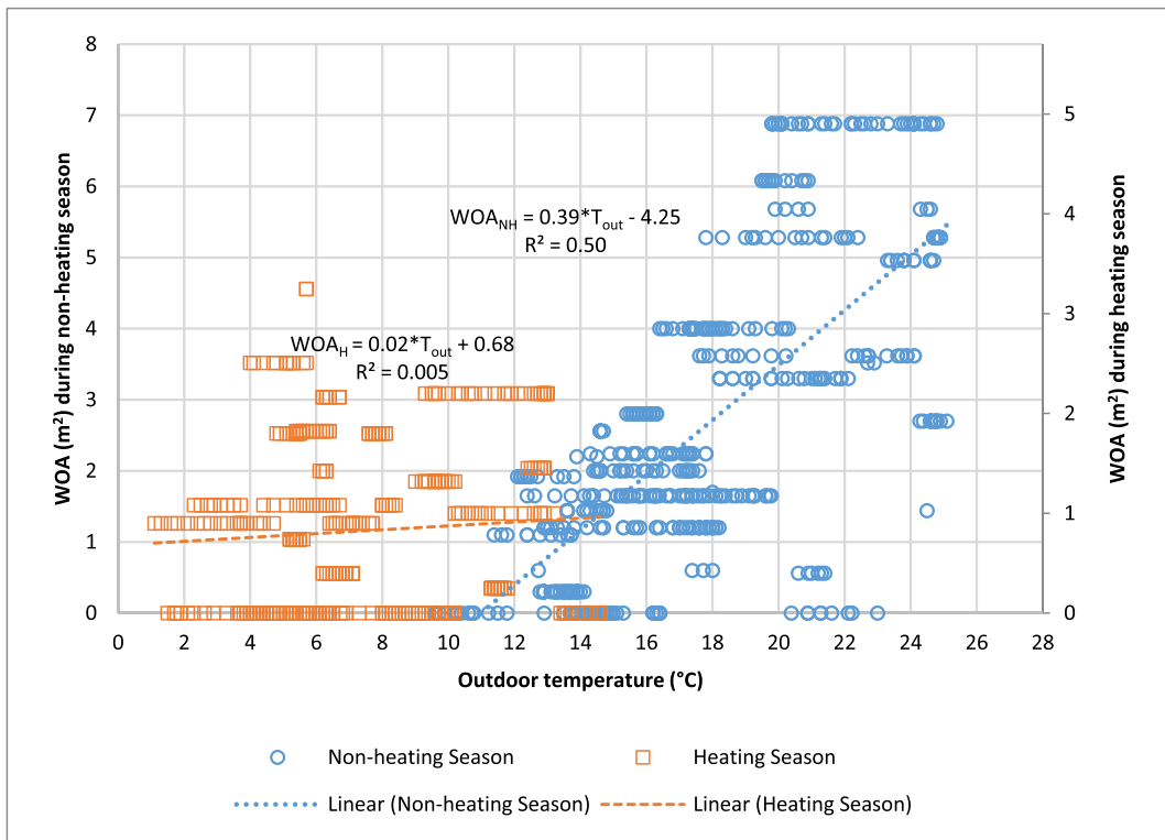
Fig. 11. Behavioural models for WOA (m 2 ) and outdoor temperature (°C).
