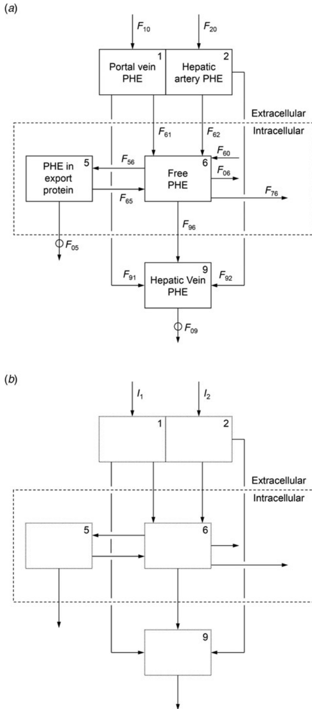
Fig. 2. Scheme for the uptake and utilization of PHE by the liver of lactating dairy cows: (a) total PHE, (b) [ 13 C] labelled PHE. The small circles in Fig. 2(a) indicate flows out of the system which need to be measured experimentally.
