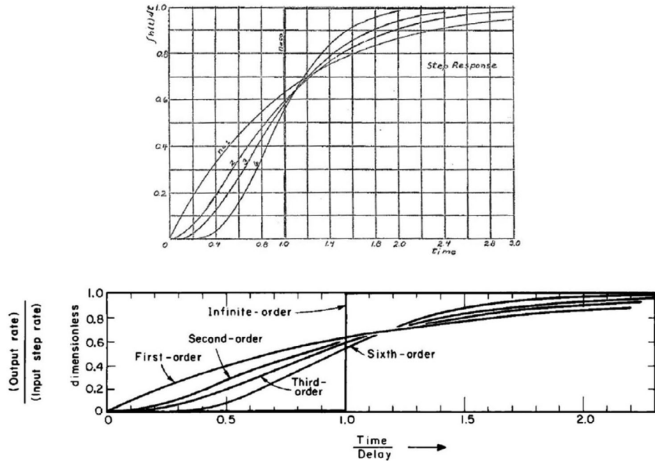
Figure 9-8 Exponential-delay responses to a unit-step rate.
