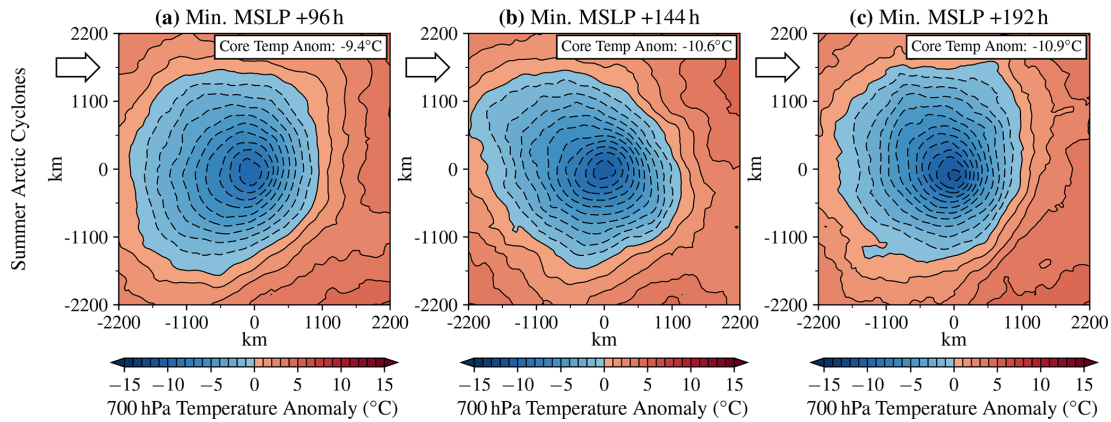
Figure 7. Horizontal 700 hPa temperature anomaly (°C) composite structure 96 h (a), 144 h (b), and 192 h (c) after the time of maximum intensity (i.e. minimum MSLP) of summer (JJA) Arctic cyclones. The large arrow indicates the direction of cyclone propagation.
