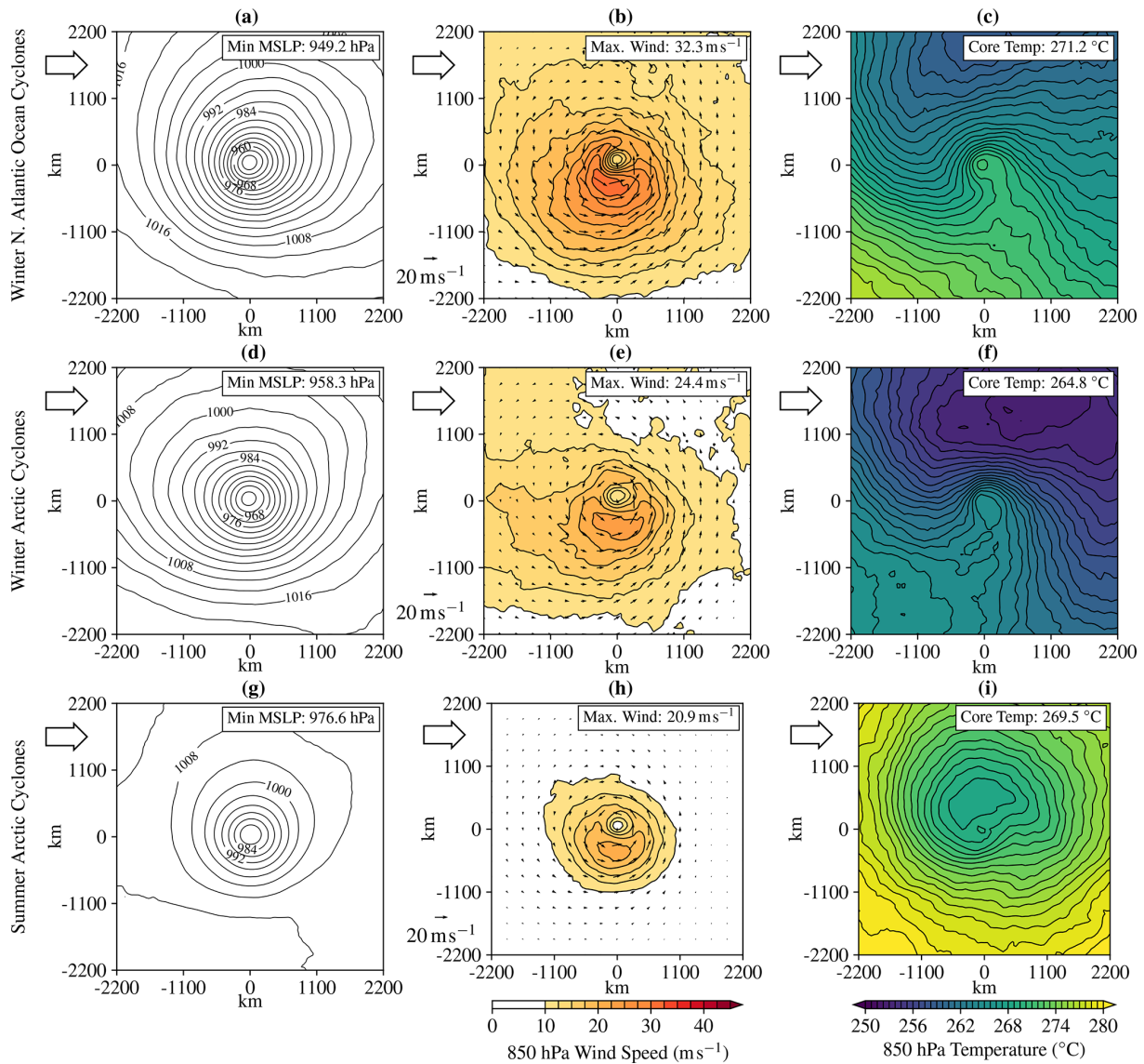
Figure 3. Horizontal mean sea level pressure (MSLP) (hPa) (a, d, g), 850 hPa earth-relative wind speed ( \text{m s}^{-1} ) (b, e, h), and 850 hPa temperature ( ^{\circ}\text{C} ) (c, f, i) composite structure at the time of maximum intensity (i.e. minimum MSLP) of winter (DJF) North Atlantic Ocean extra-tropical cyclones (a–c), winter Arctic cyclones (d–f), and summer (JJA) Arctic cyclones (g–i). The large arrow indicates the direction of cyclone propagation.
