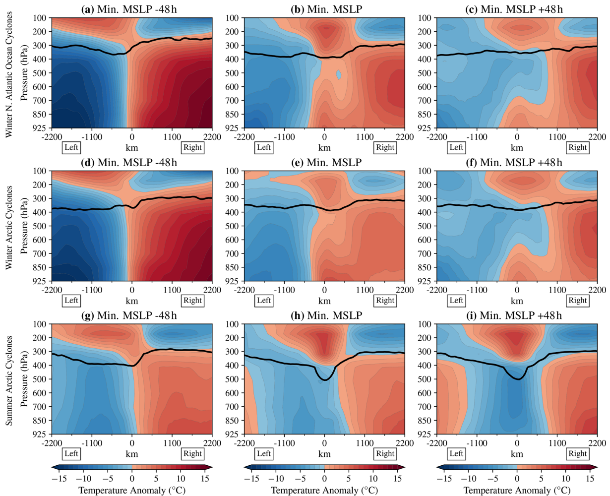
Figure 8. Vertical temperature anomaly (°C) composite of winter (DJF) North Atlantic Ocean extra-tropical cyclones (a–c), winter Arctic cyclones (d–f), and summer (JJA) Arctic cyclones (g–i) along the transect perpendicular to the cyclone propagation direction through the composite cyclone centre 48 h before the time of maximum intensity (i.e. minimum MSLP) (a, d, g), at the time of maximum intensity (b, e, h), and 48 h after the time of maximum intensity (c, f, i). The thick black contour indicates the level of the tropopause (i.e. the 2 PVU, potential vorticity units, contour). The positions (left/right) are shown relative to the cyclone propagation direction.
