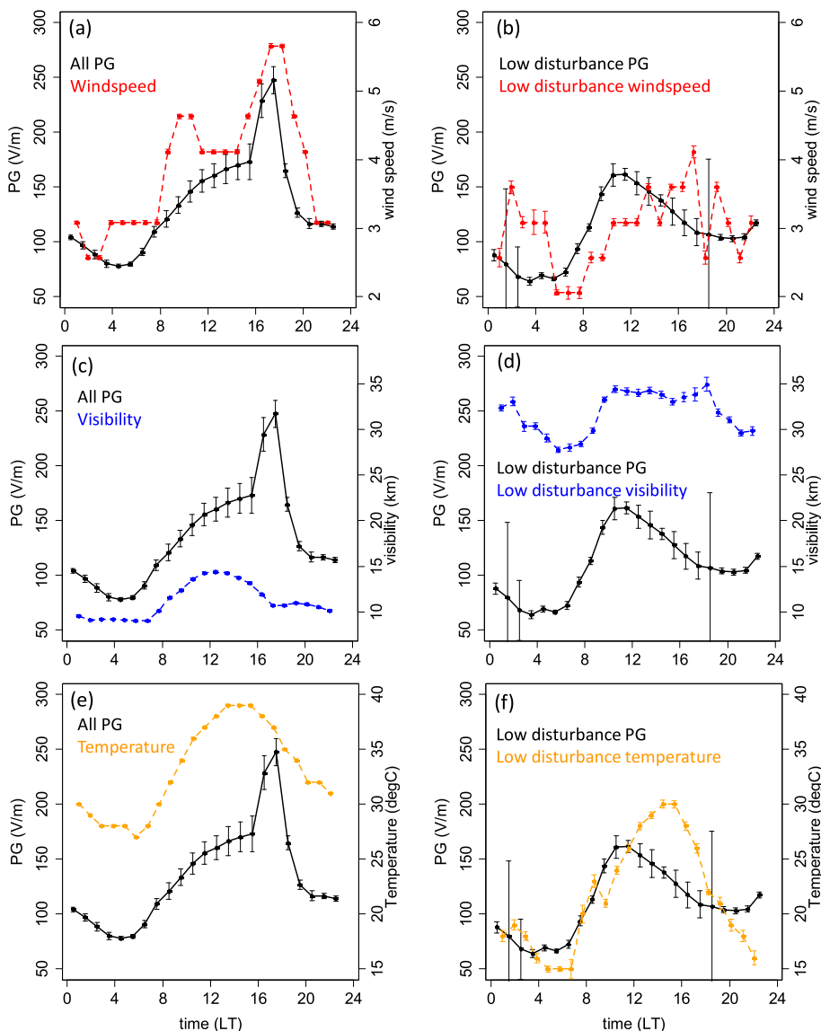
Fig. 12. Diurnal variation in PG during all conditions ((a), (c) and (e)) and low disturbance conditions ((b), (d) and (f)) (defined according to S2 in Table 1). Hourly median in 10m wind speed is shown in red, visibility in blue, and temperature in orange for all conditions ((a),(c) and (e)), and for time periods corresponding to S2 selected PG values only ((b), (d), (f)). Data points are hourly medians (based on 1 min values) and error bars are 2 standard errors on the mean. N.B. data is plotted in local time (LT), unlike in the other plots.
