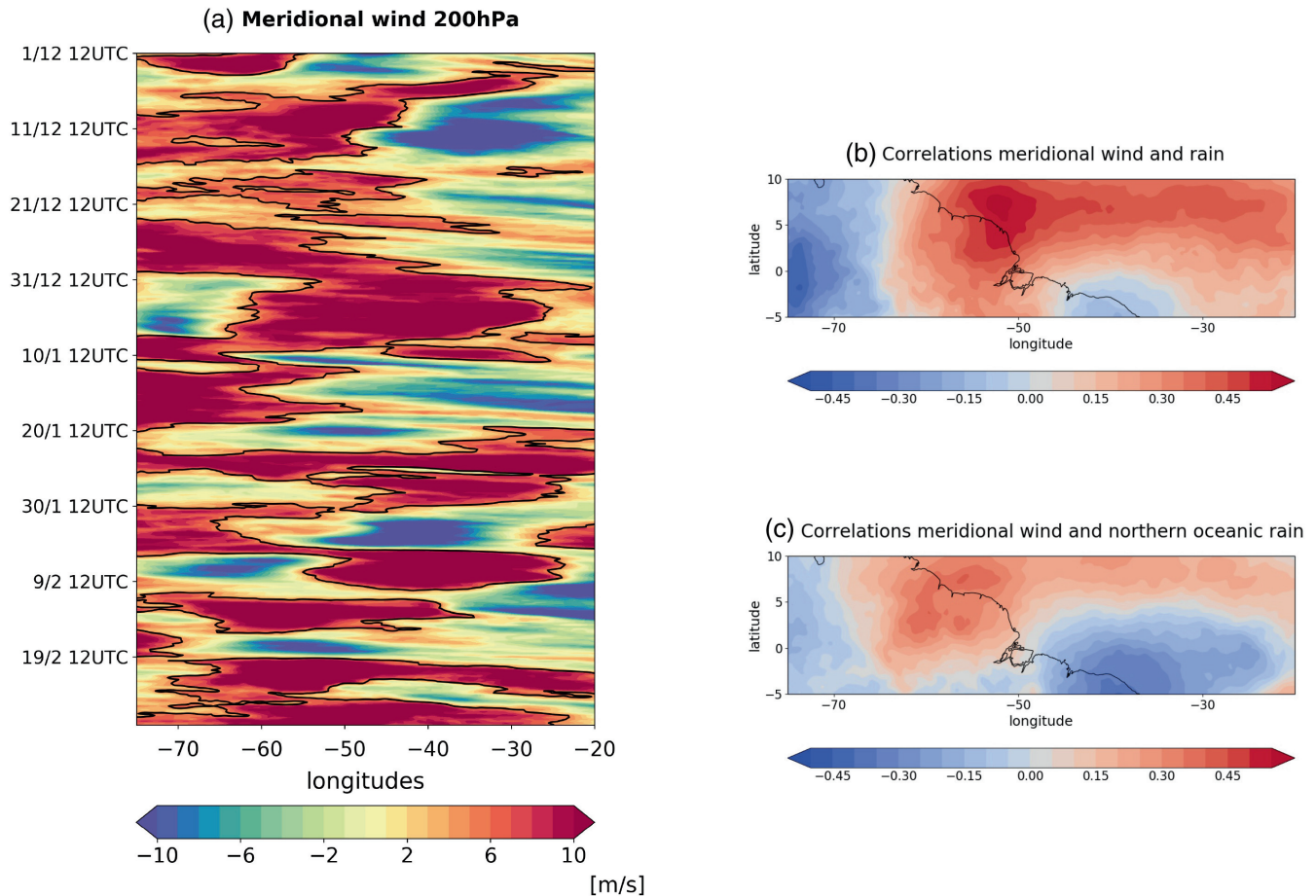
FIGURE 4 (a) Hovmöller plot of meridional wind at 200 hPa, latitudinally averaged as indicated by the black box in Figure 1a. The 5 m·s -1 contour is included. (b) Correlations between mean rainfall averaged over the box indicated in Figure 1d and meridional wind at 200 hPa for each grid box, calculated based on the boreal winter season 2019/2020. (c) Same as in panel (b), but with the rainfall averaged only over the oceanic rainband area north of the Equator (see Figure 1d), namely 0–8°N and –40 to –20 °E
