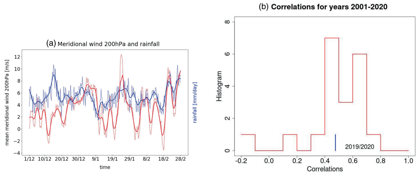
FIGURE 3 (a) Time series of mean meridional wind at 200 hPa averaged over the box indicated in Figure 1a (red dashed line) and rainfall averaged over the area indicated in Figure 1d (blue dashed line) for the boreal winter 2019/2020. The corresponding solid lines show the same data, but smoothed based on local polynomial regression fitting with span = 0.05. (b) Histogram of correlations between smoothed 200-hPa meridional wind time series and rainfall time series based on the values for the 20 boreal winter seasons 2001–2020. The value for the 2019/2020 season is indicated by a vertical blue line; it is 0.476 and below both the mean and the median of the distribution
