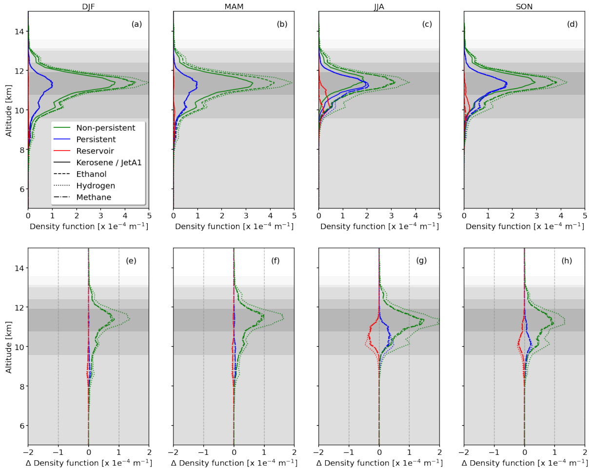
Figure 8. (a–d) Joint probability, p(\text{Rx} = \text{R}, z) , of an aircraft flying through a region that satisfies the conditions for R1-NPC (green curves), R2-PC (blue curves) or R3-R at a given altitude. The flight altitude distribution is provided by the gray shading indicating the 10, 25, 50, 75, and 90 th percentile. PDFs are shown for kerosene / Jet-A1 (solid), ethanol (dashed), hydrogen (dotted), and methane (long dashed). The four panels represent the four seasons. (e–h) Absolute differences of the PDFs with respect to kerosene / Jet-A1, given by the black, dash-dotted line.
