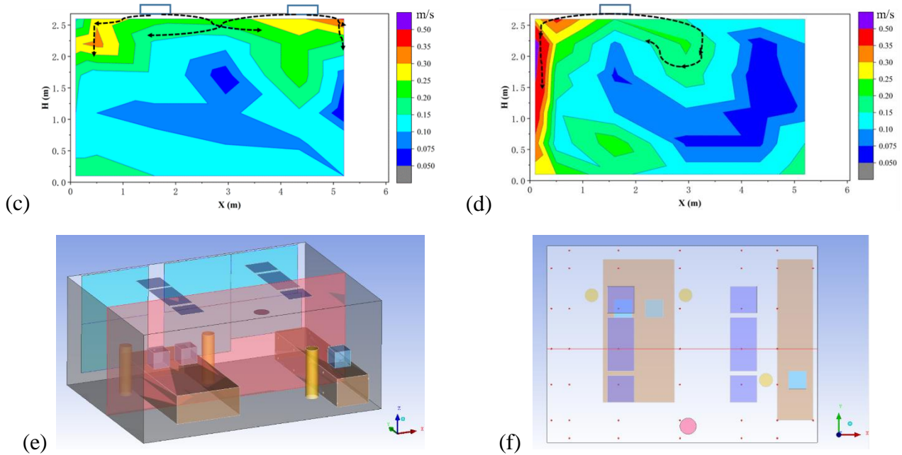
1 Fig.7: The contour plot of the air velocity in the plane below the central line of the low heat gain 2 cases, (a) O-Low-4x600; (b) O-Low-2x600; (c) O-Low-2x1200; (d) O-Low-1x1200; (e) elevations 3 of the test points; (f) plane of the test points.
