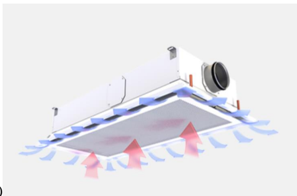
Fig. 2: The 4-way active chilled beam system design, (a) air flows, where the red arrow shows the induced room air and the blue arrow is the total supply air; (b) structural design: ① front panel, ② nozzles, ③ integrated VAV supply air valve with motorized actuator, ④ plenum, ⑤ brackets, ⑥ spigot, ⑦ frame, ⑧ connection pipes, ⑨ coil/heat exchanger.
