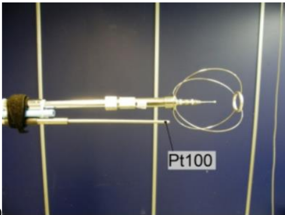
4 Fig. 3: (a) The air velocity probe (HT412) and air temperature sensor (Pt100); (b) the heights of the 5 sensors. 6
