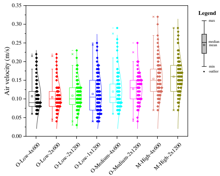
8 Fig. 6: The distribution of air velocity in the occupied zone with different chilled beam types.
