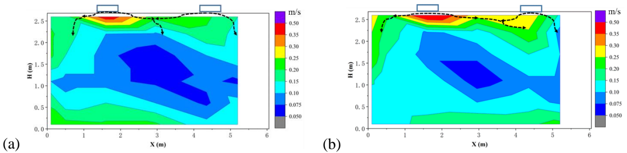
8 Fig. 6: The distribution of air velocity in the occupied zone with different chilled beam types.
