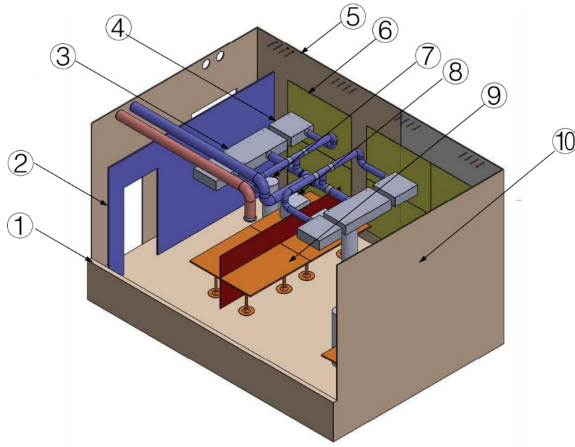
Fig. 1: Layout of the test chamber: ① observation window wall, ② door side wall, ③ 1200 chilled beam, ④ 600 chilled beam, ⑤ mock-up window wall, ⑥ electrical heating foil, ⑦ dummy (manikin), ⑧ computer, ⑨ table, ⑩ side wall.
