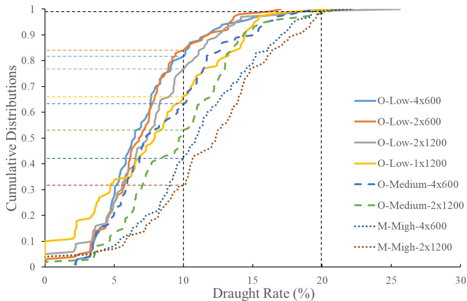
10 11 Fig.10: The cumulative distributions of draught rate (DR) in the occupied zone with different chilled 12 beam types. 13
