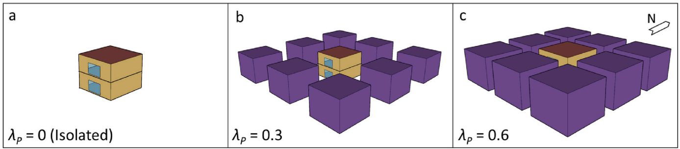
Fig. 2. A reference building (8 m (L) × 8 m (W) × 6.4 m (H)) is simulated using EnergyPlus in: (a) a rural (isolated) site, and in neighbourhoods with a plan area fractions \lambda_p = (b) 0.3 and (c) 0.6.
