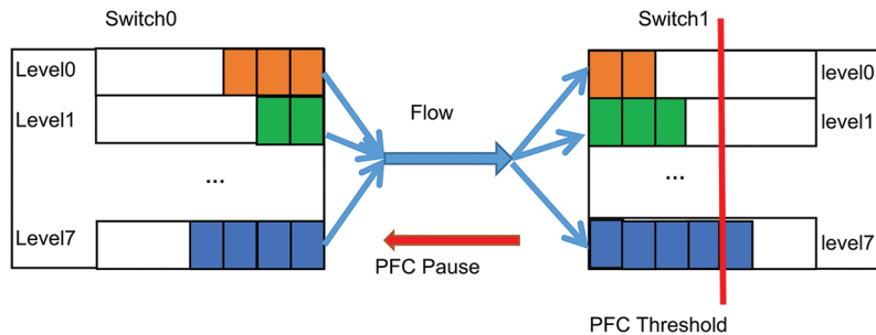
Figure 1: PFC mechanism
