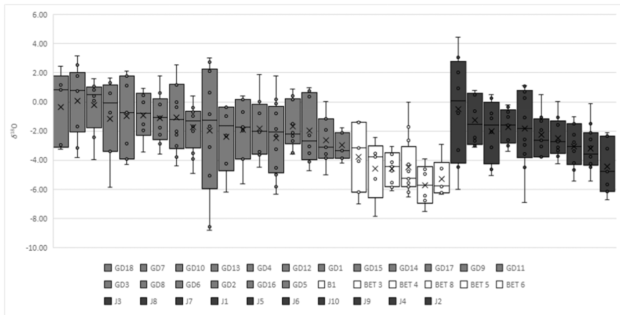
Fig. 11. Boxplot of the \delta^{18}\text{O} values (all sequences with >5 datapoints included, in order of descending mean value), light grey = Ganj Dareh, white = Bestansur, dark grey = Jarmo.
