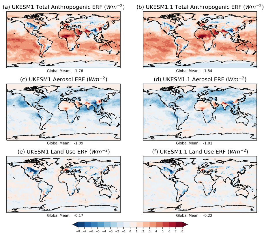
Figure 17. Comparison of the anthropogenic effective radiative forcing (ERF) in (a, c, e) UKESM1 and (b, d, f) UKESM1.1. (a, b) The total anthropogenic ERF, (c, d) aerosol ERF and (e, f) land use change ERF. The ERFs are calculated for the year 2014 relative to an 1850 preindustrial control, following Pincus et al. (2016).
