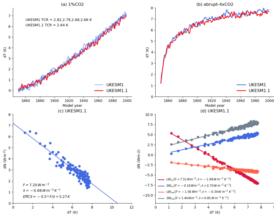
Figure 18. Evolution of the global annual mean surface air temperature change in the (a) 1pctCO 2 and (b) abrupt-4×CO 2 simulations from UKESM1 (blue line) and UKESM1.1 (red line). (c) Regression of the change in net downward radiative flux, N , at the TOA radiation against the change in surface temperature for UKESM1.1. Panel (d) is the same as panel (c) but for the individual SW and LW clear-sky and cloudy-sky components.
