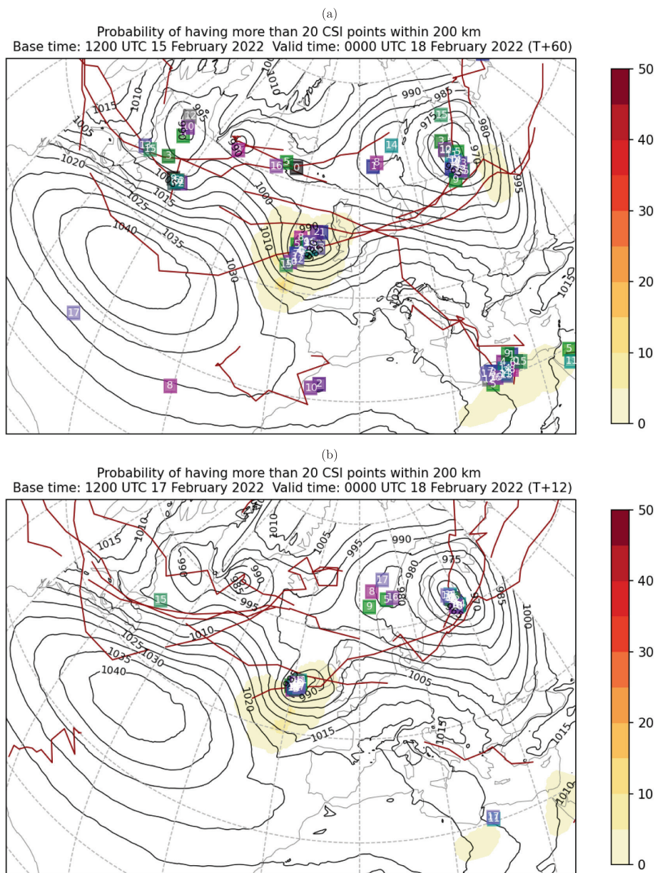
Figure 4. Ensemble-based probability of sting-jet precursor for greater than 20 CSI points (on a 0.5^\circ \times 0.5^\circ grid) within 200 km (shaded), valid at 0000 UTC on 18 February, with data from the global operational UK Met Office forecasts initialised at (a) 1200 UTC on 15 February and (b) 1200 UTC on 17 February. The conditional symmetric instability (CSI) points are all within 1000 km of a cyclone centre and constitute sets whose centroids are within 700 km of a cyclone centre in the cloud head sector and with moisture available for the instability to be released. Overlain are the cyclone tracks of all the storms identified during the period (dark red lines) and the mean sea-level pressure (black contours every 5 hPa) at the verification time from the control ensemble member. The squares along the tracks indicate the locations of the cyclone centres at the verification time colour-coded and numbered by ensemble member.
