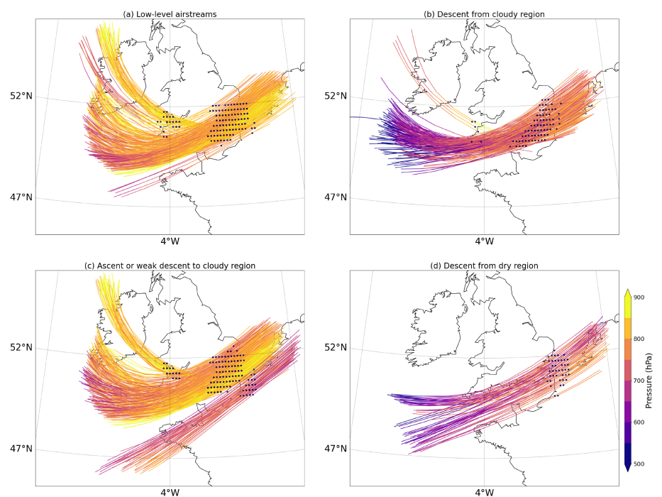
Figure 3. Lagrangian trajectories starting at 1200 UTC on 18 February (forecast start time 0600 UTC), running backward for six hours and forward for two hours and shaded by air pressure. Starting points are defined by wind speed >42\text{ms}^{-1} and pressure between 950 and 800hPa for panel (a) and between 950 and 700hPa for other panels. Horizontal starting domain is 4^{\circ}\text{W} – 3^{\circ}\text{E} and 50 – 53^{\circ}\text{N} for all panels. Additional conditions (listed in the text) applied in panels (b–d) to isolate and characterise the airstreams are summarised in the panel titles.
