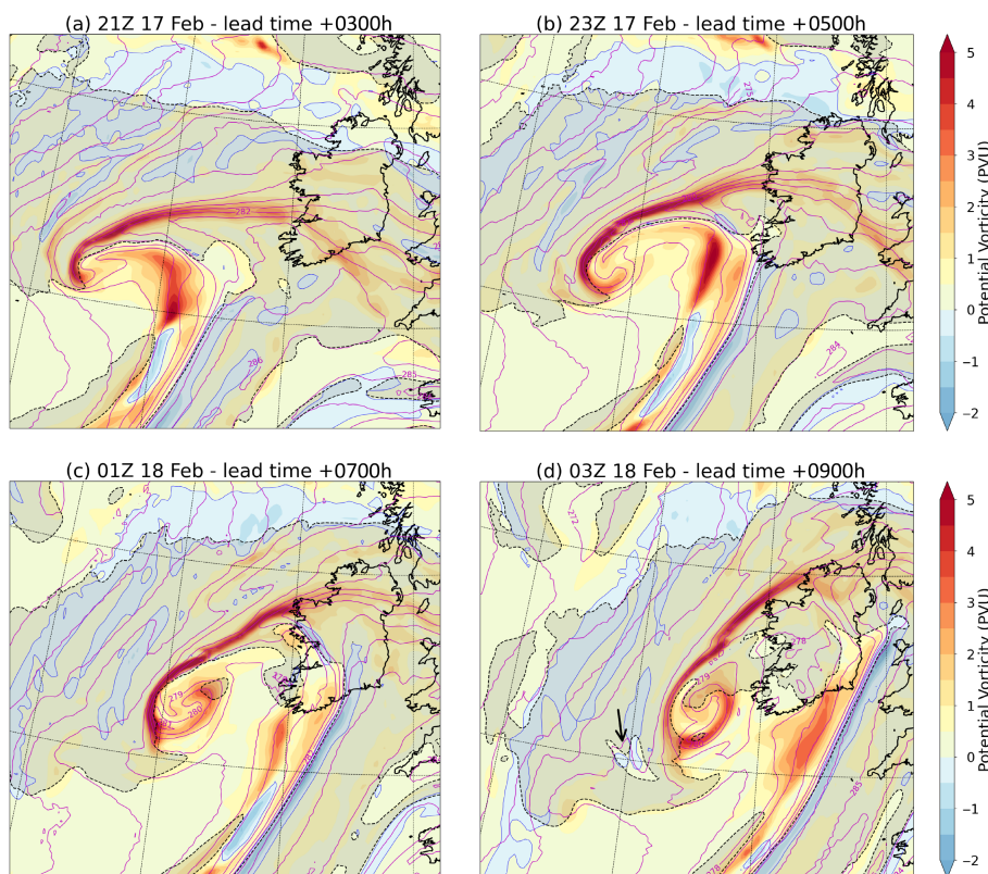
Figure 1. Potential vorticity (shading, PVU), wet-bulb potential temperature (magenta contours, every 1K) and relative humidity with respect to ice (dashed black contours, 80%, and semi-transparent grey shading, 80% and above) from Met Office global operational forecasts initialised at 1800 UTC on 17 February (valid and lead times indicated on top of each panel). All quantities are displayed at 700hPa. The black arrow in panel (d) indicates the location of the cloud hole described in the text.
