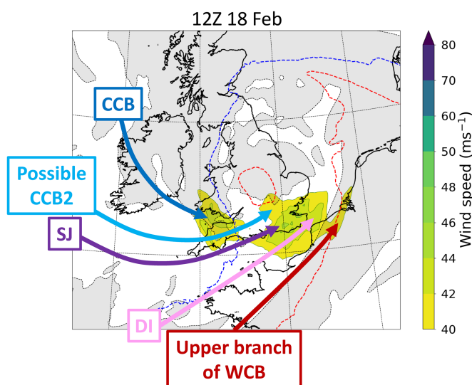
Figure 4. Schematic, adapted from Figure 2(e), illustrating the airstreams associated with strong winds over southeast England and nearby regions at 1200UTC on 18 February. The schematic includes horizontal wind speed at 850hPa (shading, \text{ms}^{-1} ), \theta_w at 850hPa (dashed contours, red for 280K and blue for 277K), and relative humidity with respect to ice at 700hPa (grey shading, >80%).
