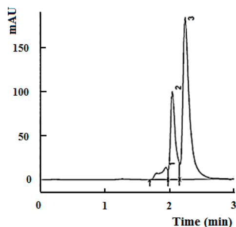
Figure 13. Chromatograph of solution after 45 min hydrogel immersion in saline solution, peaks: hydrochloride chitosan (1), apple pectin (2), cisplatin (3).
