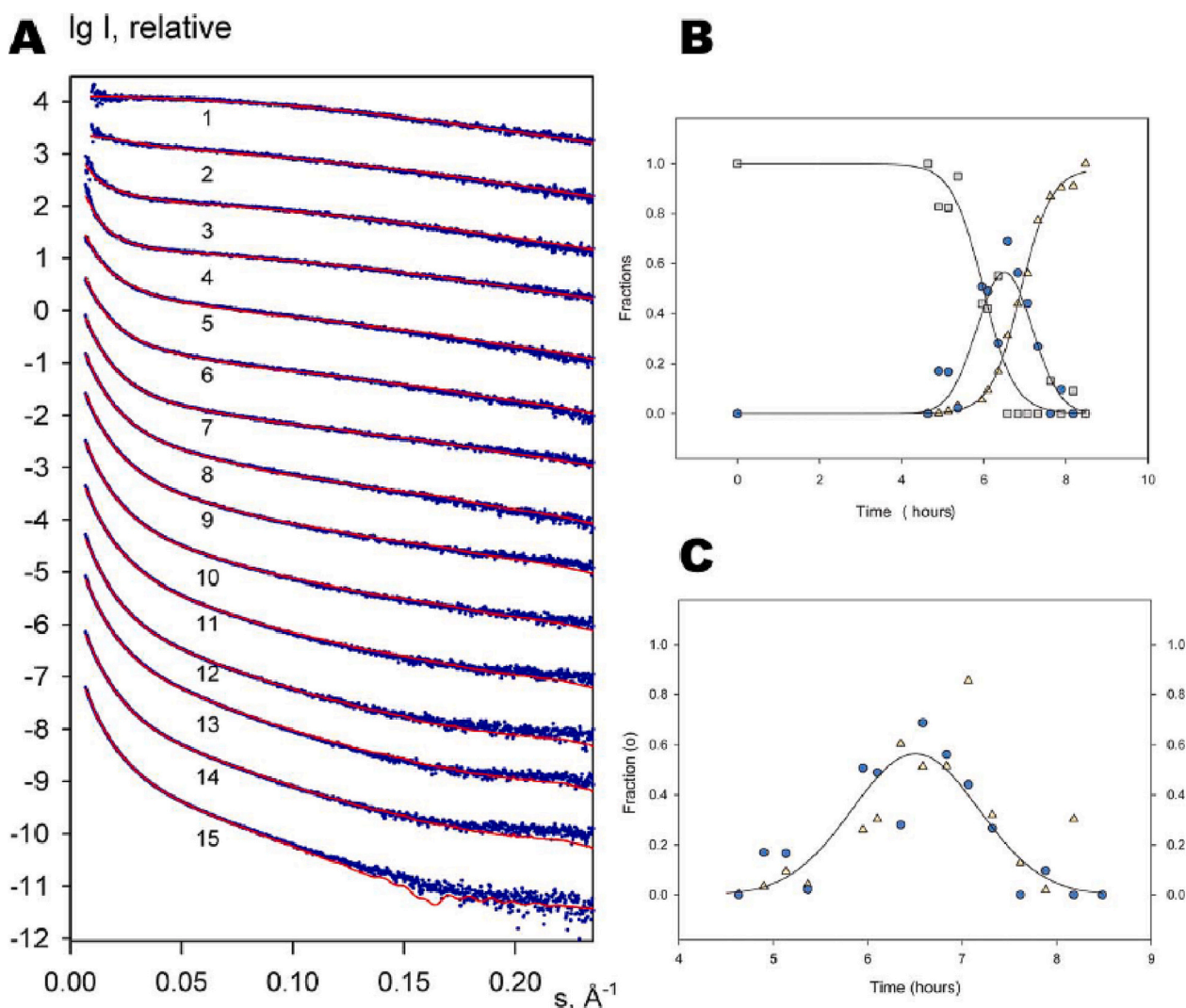
Fig. 11. A) SAXS data for insulin aqueous solution (pH 2, with NaCl, T = 45 °C) as a function of time (in h, the successive curves labelled 1 to 15 are displaced by one logarithmic unit for clarity). Blue dots: experimental data, red lines: fits for the three-component mixtures (for the bottom curve, a fit from an ab initio shape model obtained for fibrils is displayed). B) Relative fractions of components present. Grey squares: insulin monomer, blue circles: helical oligomer, beige triangles: fibril. C) Comparison of oligomer fraction (blue circles and fitted curve) with rate of formation (first derivative) of fibril component (beige triangles). Reproduced from ref [166].
