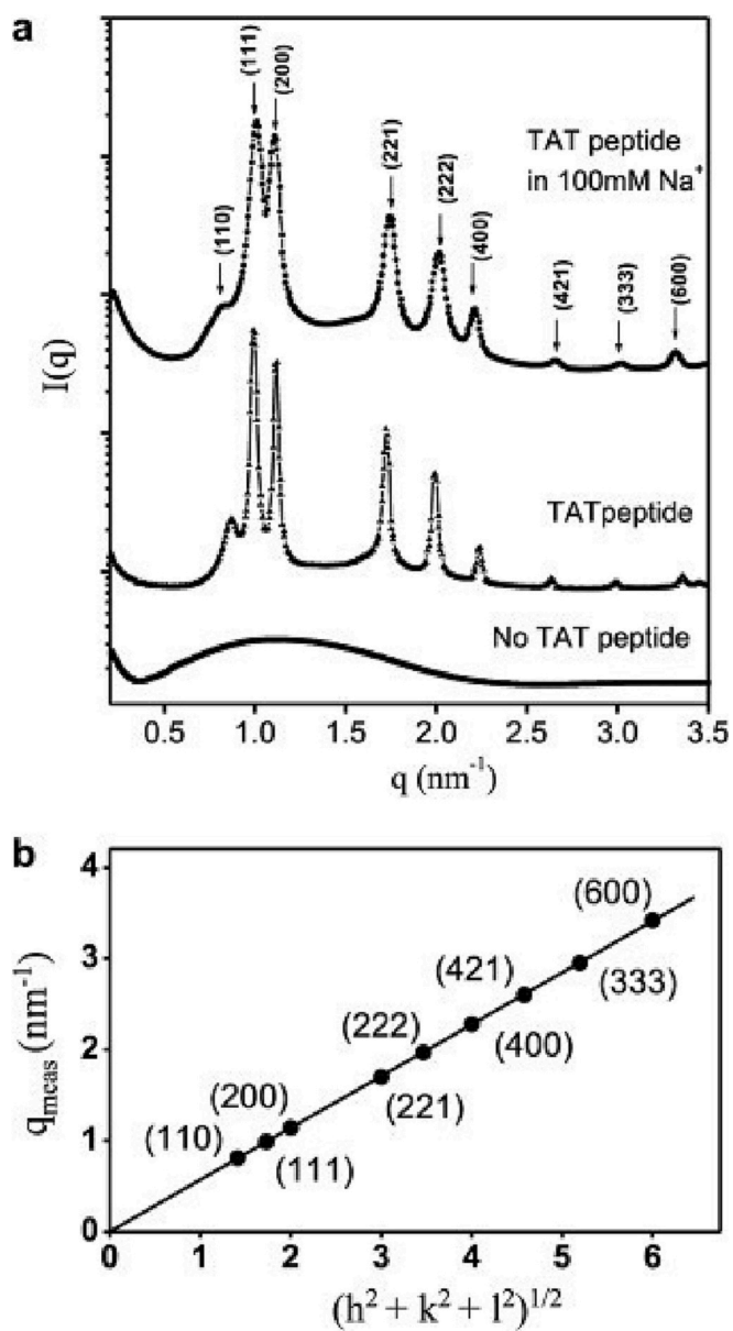
Fig. 8. SAXS from the TAT cell-penetrating peptide with a mixed zwitterionic/anionic lipid system, (a) SAXS data showing Bragg peaks induced by the peptide causing curvature of the lipid membrane and bicontinuous cubic phase formation, (b) Indexation of the peaks indicates a 'double diamond' Pn\bar{3}m structure with lattice parameter a = 10.97 nm, (c) Schematic of the corresponding bicontinuous cubic phase. From reference [154].
