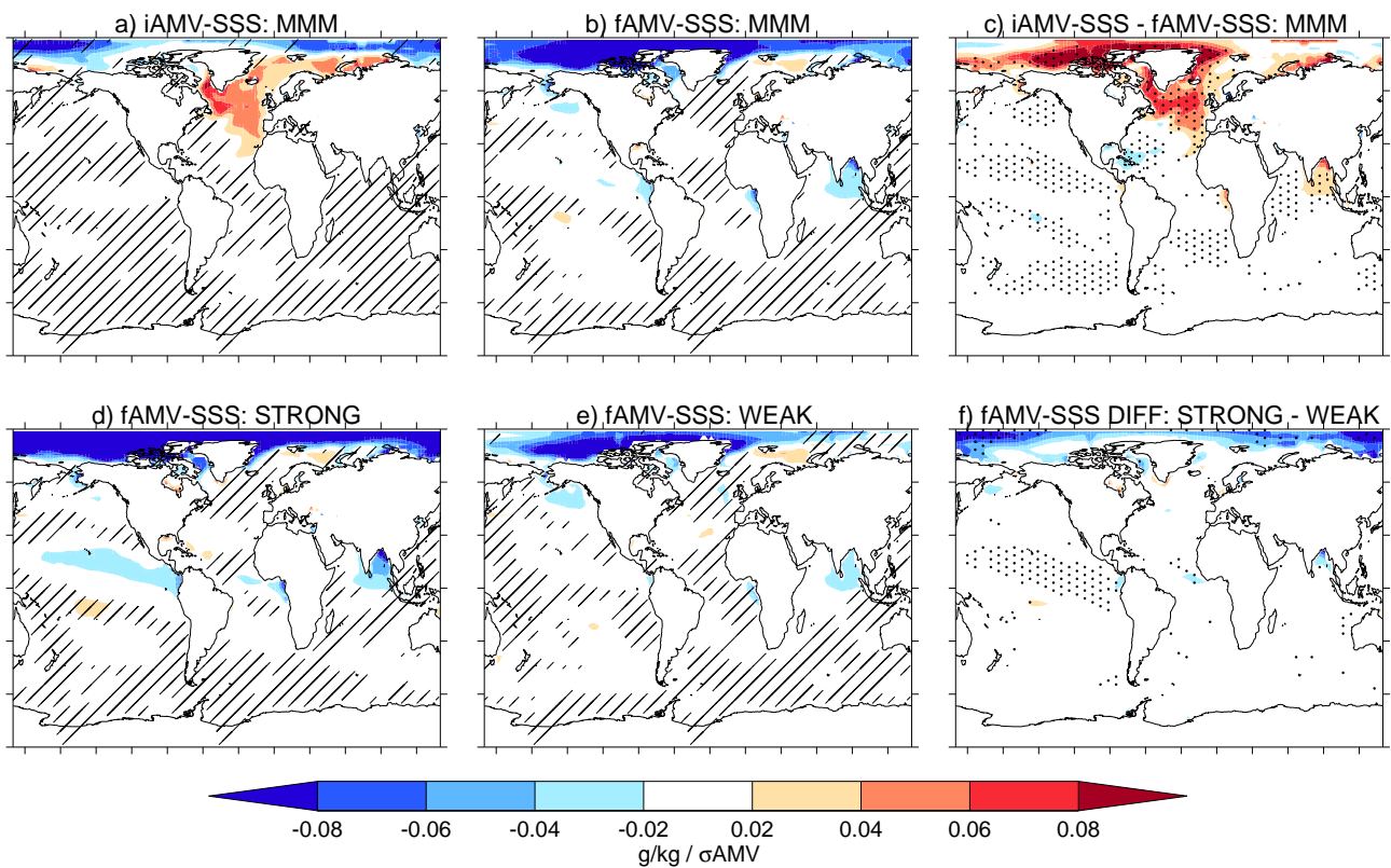
Figure S5: Shows the same as figure S4 but now for the relationship between AMV and sea surface salinity (AMV-SSS) across the internal and external components of AMV. Note this is the same as figure 7 in the main paper, but now for AMV BM rather than AMV-Glob.
