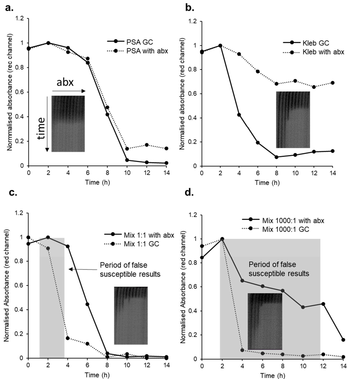
Figure 6. False susceptibility when a susceptible coliform ( Kleb ; Klebsiella spp.) commensal organism in is higher abundance than a resistant mastitis-causing pathogen (PSA; Pseudomonas spp.) in the presence of ciprofloxacin ( n = 3 ). Inset images show the full MIC test strip with 9 antibiotic concentrations, capillary 1 indicates 0.5 mg/L ciprofloxacin with decreasing in \log_2 dilutions from left to right plus no antibiotic—termed growth control (GC) at the far right. Time course images indicate 18 h incubation time. Bacterial growth results in resazurin conversion and decrease in absorbance. (a) Growth kinetics of the resistant pathogen alone with and without ciprofloxacin at the MIC for the commensal (0.125 mg/L, capillary 3); GC indicates growth control without the presence of antibiotics. (b) Growth kinetics of commensal with and without ciprofloxacin at the MIC for the commensal (0.125 mg/L). (c) Pathogen and commensal at equal inoculum densities with and without ciprofloxacin at the MIC of the commensal (0.125 mg/L). Period of false susceptibility present. Total plate count is 8 \times 10^4 CFU/mL (d) Growth kinetics of the resistant pathogen spiked at 10^4 CFU/mL and susceptible commensal at 10^7 CFU/mL, total plate count is 3 \times 10^6 CFU/mL, with and without ciprofloxacin at the MIC of the commensal (0.125 mg/L). Period of false susceptibility present. Colour change caused by growth of the resistant pathogen in the presence of antibiotics not evident until after 10 h. abx = antibiotics.
