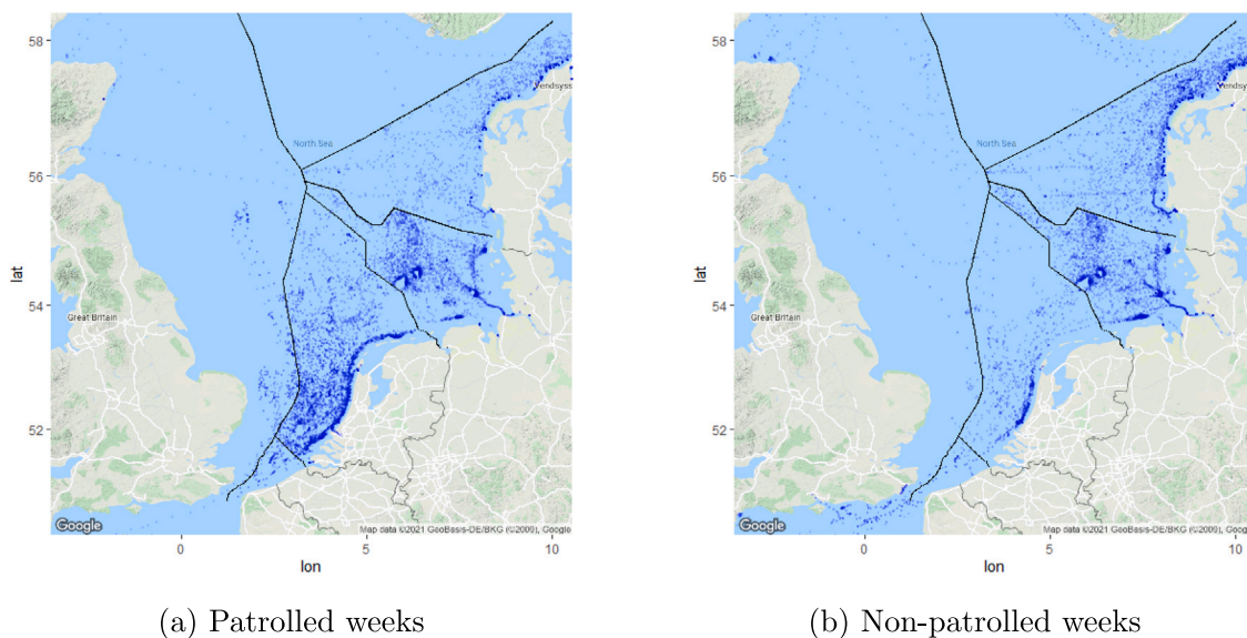
Fig. 17. Dutch, German and Danish inspection vessels' navigation signals.
