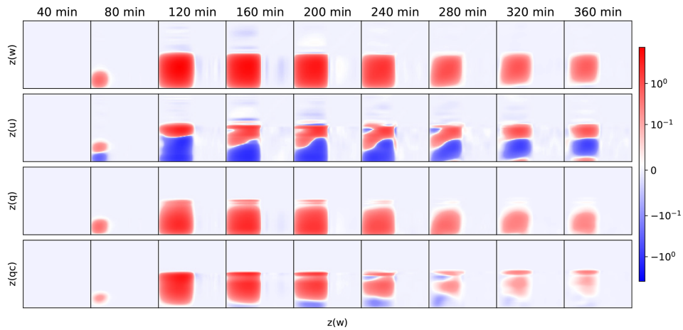
Figure 5. Evolution of a selection of normalised vertical covariances in the convection zone ( x = 148.5 km) at times between 40 and 360 min. The rows are for w – w , u – w , q – w , and q_c – w covariances. In each plot of p_1 – p_2 covariances, the y axis is for p_1 and the x axis is for p_2 , and the surface is at the bottom left of each square. Red (blue) indicates positive (negative) covariances according to the logarithmic scale shown.
