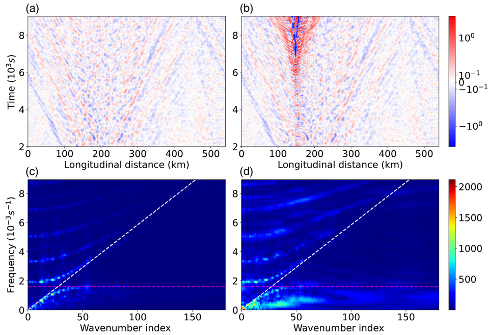
Figure 4. Vertical wind in the longitude–time (a, b) and wavenumber–frequency (c, d) domains for level 30 in the model (7.7 km height). The left panels are for dry ABC, and the right panels are for Hydro-ABC. The initial conditions of u , v , w , \tilde{\rho}' , and b' are identical for ABC and Hydro-ABC, and the additional initial conditions for q and q_c are the same as those used in Fig. 2. In (c) and (d), the horizontal dashed lines are each at frequency A/(2\pi) (the pure gravity wave frequency), and the sloped dashed lines each have gradient df/dn = L^{-1}\sqrt{BC} (the pure sound wave speed), where f is frequency (the y axes), n is the wavenumber index (the x axes), and L is the length of the domain, 540 \times 10^3 m.
