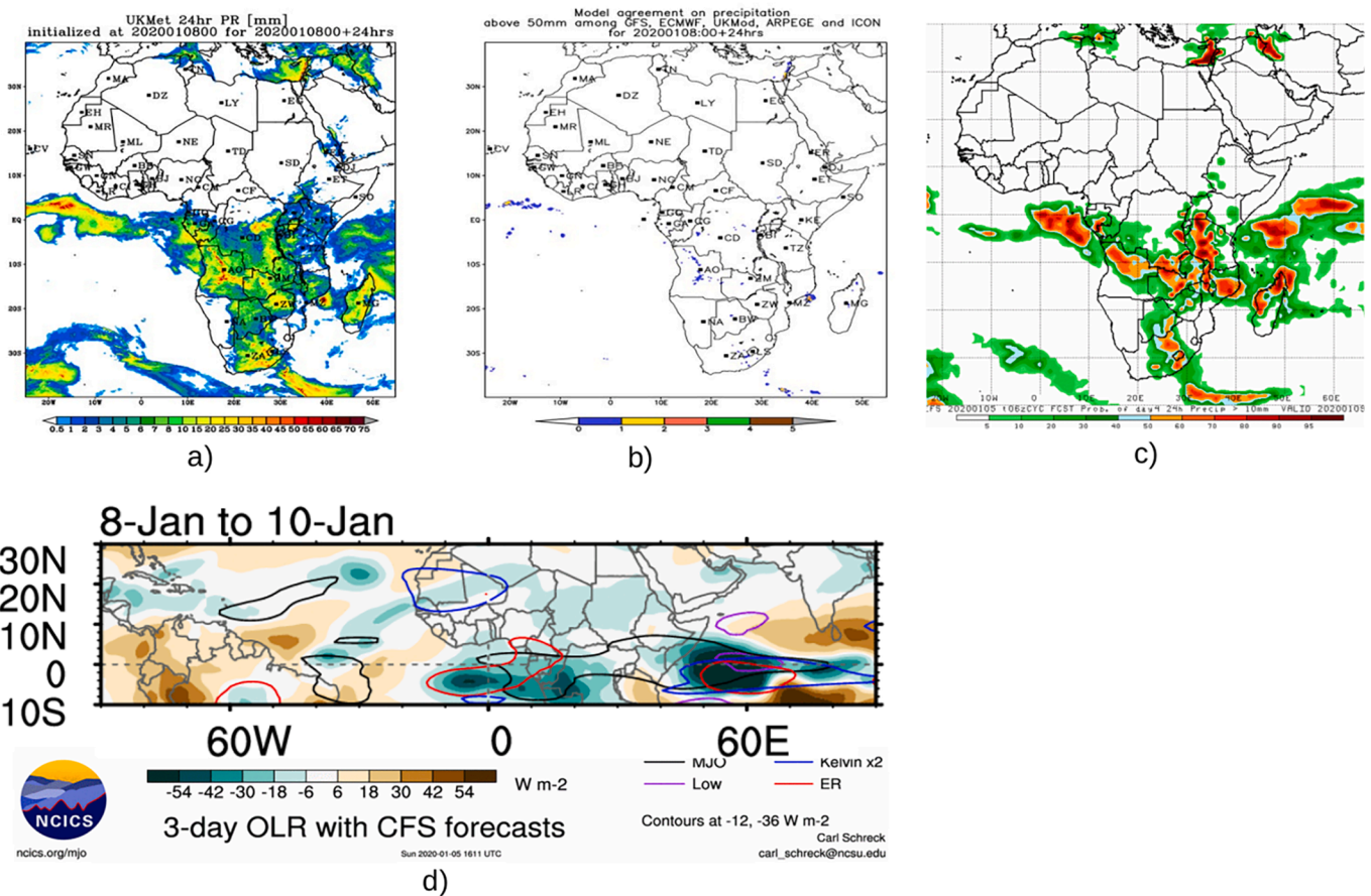
Fig. 6. Selected products used for daily forecasting on the 8th January 2020 and valid for 9th January 2020 including: a) UKMO precipitation (mm) forecast from ACMAD, b) model agreement between precipitation forecasts (GFS, ECMWF, ARPEGE, UKMet and ICON) of surpassing a threshold of 50 \text{ mm day}^{-1} , c) NOAA (NCEP) probability of precipitation greater than 10 mm and d) CFSv2 forecasts and equatorial waves and 3-day OLR anomalies ( \text{W m}^{-2} ) ending 10 January 2020.
