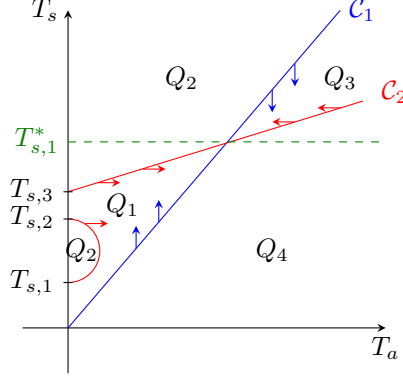
FIGURE 9. In the phase space we represent the case of one equilibrium point (2^{-1/4}T_{s,1}^*, T_{a,1}^*) , which is solution of (6.1), and therefore intersection of the curves \mathcal{C}_1 : T_s = 2^{1/4}T_a and the one defined by the set \mathcal{C}_2 = \{(T_a, T_s) \in \mathbb{R}^2 : -\sigma_B|T_s|^3T_s + \varepsilon_a\sigma_B|T_a|^3T_a + q\beta_s(T_s) = 0\} . In particular, here we consider the case of three solutions of the equation \sigma_B T_s^4 = q\beta_s(T_s) . We subdivide the set \mathcal{Q} = \{(T_a, T_s) : T_a > 0, T_s > 0\} in the subsets \mathcal{Q}_1 , \mathcal{Q}_2 , \mathcal{Q}_3 and \mathcal{Q}_4 . We describe with arrows the behaviour of the vector field on the boundaries of \mathcal{Q}_1 , \mathcal{Q}_2 , \mathcal{Q}_3 and \mathcal{Q}_4 .
