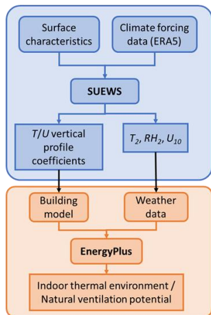
Fig. 3. Overview of the SUEWS-EnergyPlus workflow integration (Tang et al., 2021).
