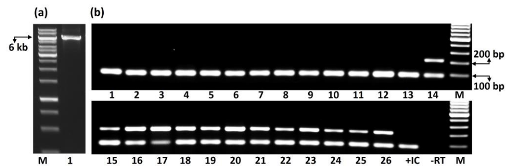
Figure 4. Agarose gel electrophoresis. (a) RT-PCR amplification of the complete genome of cacao Polerovirus virus (CaPV) from RB37. (b) Multiplex RT-PCR-based assay for testing of CaPV in the International Cocoa Quarantine Centre, Reading (ICQC-R) germplasm. A 212 bp fragment of CaPV and a 90 bp fragment of internal control [cacao ACP1 gene (LOC18599903)] were amplified from accessions RB 46 [BRA] (1), RB 49 [BRA] (2), RIM 189 [MEX] (3), EET 95 [ECU] (4), PMCT 93 (5), ARF 12 (6), PA 169 [PER] (7), CC 252 (8), CC 137 (9), EET 183 [ECU] (10), UF 712 (11), CRIOLLO 21 [CRI] (12), APA 5 (13), BE 8 (14), C SUL 3 (15), EET 387 [ECU] (16), BE 5 (17), RB 37 [BRA] (18), RB 43 [BRA] (19), RB 48 [BRA] (20), BE 2 (21), CAS 3 (22), CRIOLLO 17 [CRI] (23), GU 139/A (24), ARF 2 (25) and TSH 1188 (26). Letter M denotes the lanes loaded with 1 kb (a) or 100 bp size marker (b).
