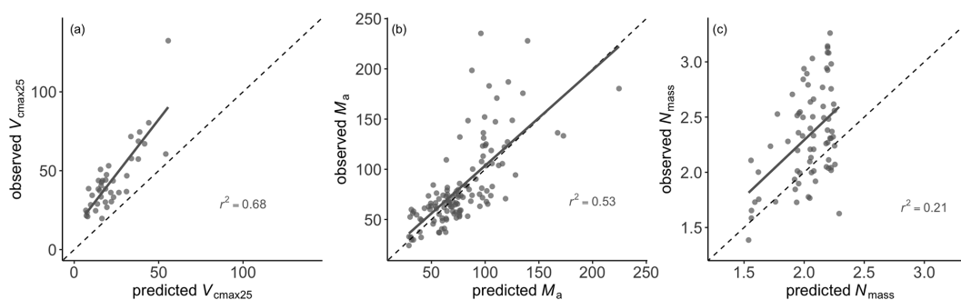
Figure 6. Optimality-based predictions versus observations of leaf traits at the site level. Grey lines are ordinary least-squares regressions. The black dashed line is the 1 : 1 line.
