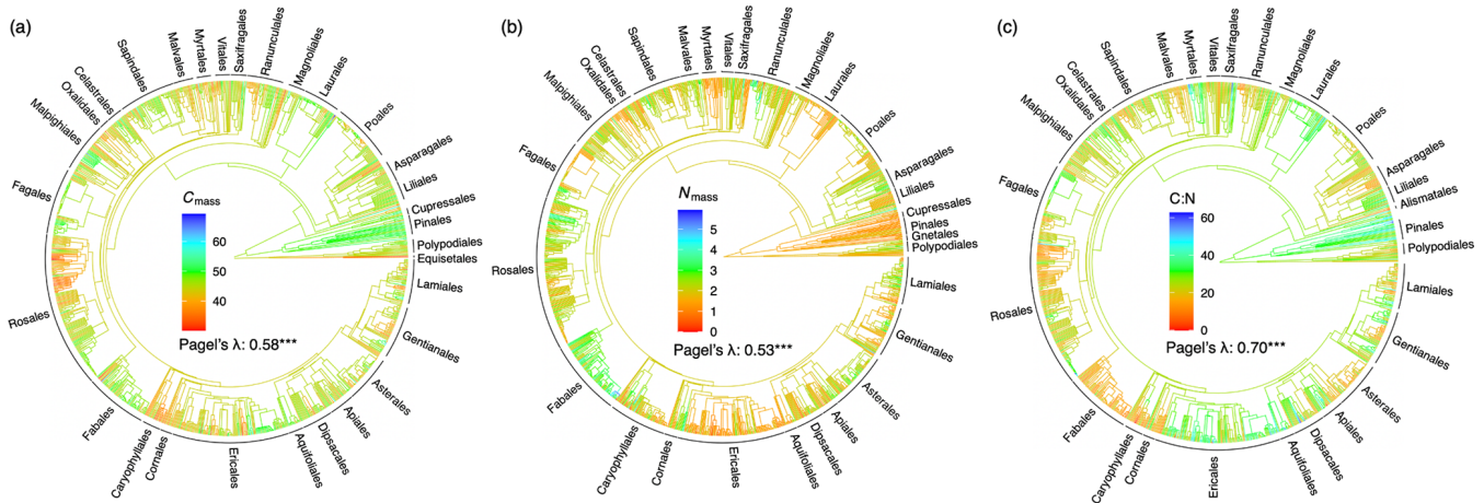
Figure 1. Phylogenetic tree and signal for (a) leaf carbon content (%), (b) nitrogen content (%), and (c) carbon-to-nitrogen ratio. The red-to-blue colours of phylogenetic trees indicate low to high trait values. The phylogenetic signal is indicated by a statistic metric of Pagel’s \lambda with its significance level (***) p < 0.001 . Orders with more than five species in the data set are labelled.
