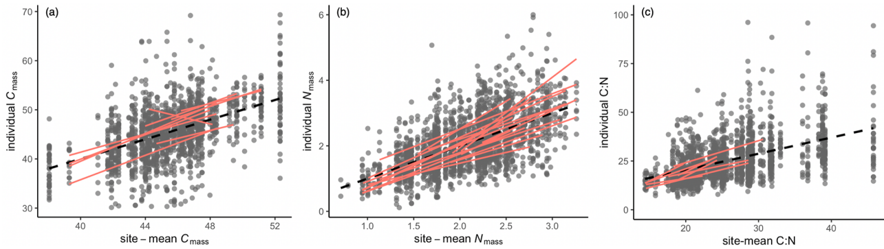
Figure 3. Distribution of site-mean trait values and within-species regression lines for leaf stoichiometric traits. The black dots are individuals, and black dashed line is the regression of all individuals with slope equal to 1 by definition. The red lines represent significant regressions within species that were sampled at more than five sites.
