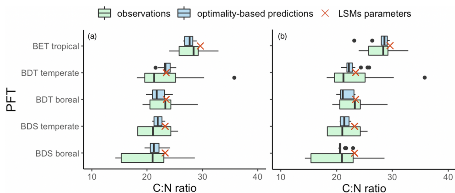
Figure 7. Comparison of observed and predicted C : N ratios with target values in LSMs. The blue boxes represent predicted C : N ratios using observed C_{\text{mass}} (a) and using constant mean C_{\text{mass}} (b). The green boxes represent observed C : N ratios. Red crosses show target values in LSMs (adopted from CLM4).
