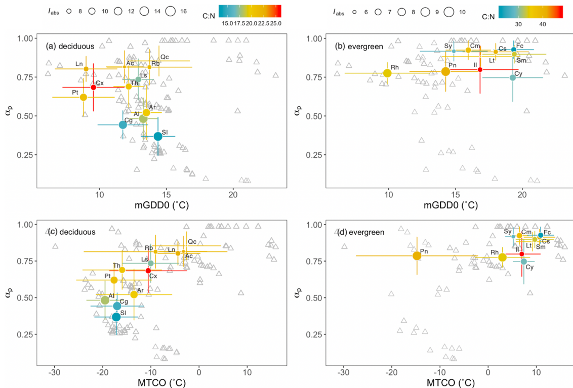
Figure 2. Optima and tolerances of major genera in climate space. \alpha_p is a moisture index, mGDD0 is the mean temperature during the thermal growing season, MTCO is the mean temperature of the coldest month, and I_{abs} is the leaf-area-index-weighted photosynthetic photon flux density. Colours of circles represent the values of the leaf C : N ratio and the sizes of circles represent I_{abs} . The grey triangles are sampling sites. Also shown are abbreviated names of genera: Ac, Acer ; Al, Allium ; Ar, Artemisia ; Cg, Caragana ; Cx, Carex ; Ls, Lespedeza ; Ln, Lonicera ; Pt, Potentilla ; Qc, Quercus ; Rb, Rubus ; Sl, Salsola ; Th, Thalictrum ; Cm, Camellia ; Cs, Castanopsis ; Cy, Cyclobalanopsis ; Fc, Ficus ; Il, Ilex ; Lt, Lithocarpus ; Pn, Pinus ; Rh, Rhododendron ; Sm, Smilax ; Sy, Symplocos .
