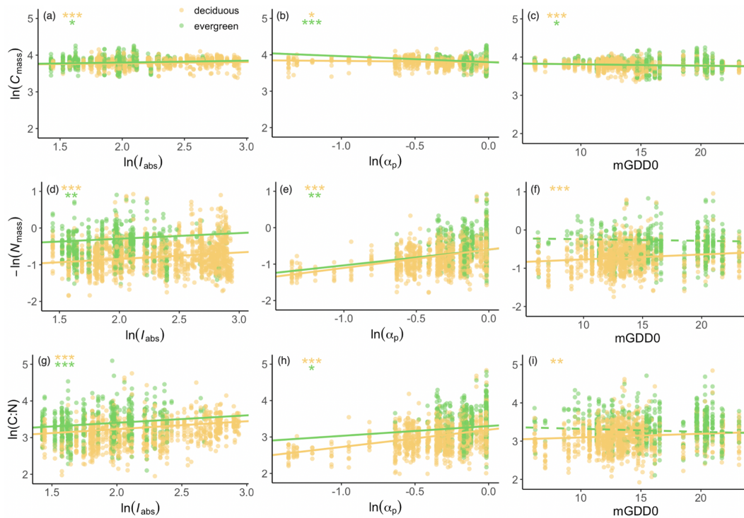
Figure 4. Empirical partial relationships between leaf traits and climate. I_{abs} is the leaf-area-index-weighted photosynthetic photon flux density, \alpha_p is a moisture index, and mGDD0 is the mean temperature during the thermal growing season. Yellow dots: deciduous species; green dots: evergreen species. The N_{mass} scale is inverted, so that the slopes of the regression lines in panels (a)–(c) and (d)–(f) should add up to the slopes in panels (g)–(i). The significance of each regression is listed in the panels. *** p < 0.001 ; ** p < 0.01 ; * p < 0.05 .
