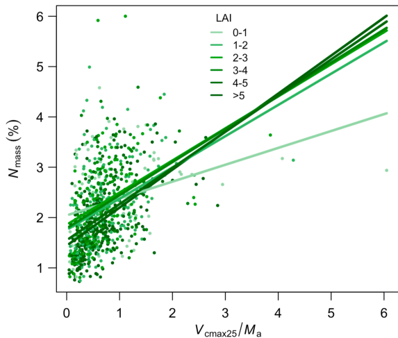
Figure 5. The relationship between N_{\text{mass}} and V_{\text{cmax}25}/M_a along the leaf area index (LAI) gradient. Colour saturation represents different levels of LAI. Lines are separate regressions for sites within each LAI bin.
