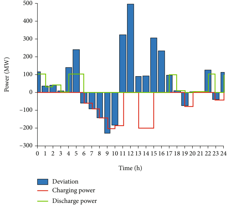
FIGURE 27: Application of energy storage in scenario 1 (Nov).
