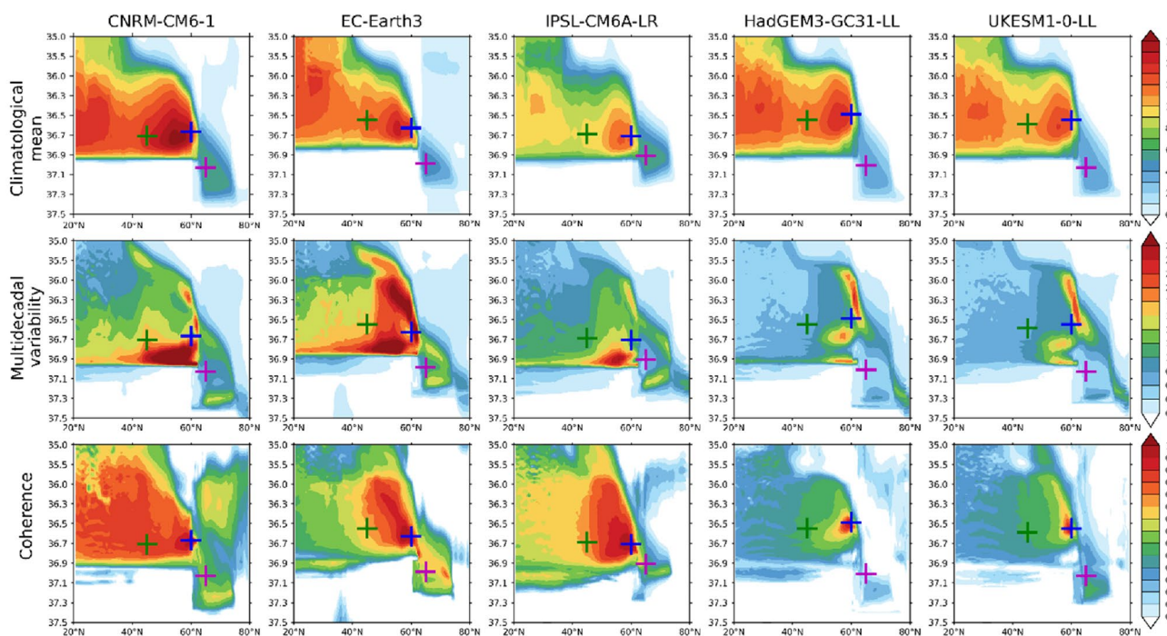
Fig. 2 Mean state, multidecadal variability, and coherence of the annual mean AMOC stream function ( Sv ) as a function of density ( \Sigma_2 ; y-axis; kg\ m^{-3} ) and latitude (x-axis). The top row shows the climatological mean. The second row shows the standard deviation of 15-year running mean of annual mean AMOC. The third row shows
