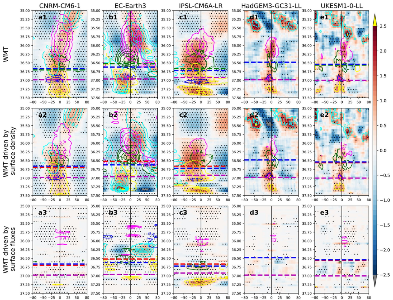
Fig. 9 Density space WMT anomalies associated with low-frequency (15-year running mean) AMOC45. (a1–e1) regression ( Sv Sv^{-1} ) of WMT onto AMOC45. Colours for WMT integrated over the broad SPNA region, while contours show WMT anomalies for different sub-sea regions: cyan for the Arctic, yellow for the GIN Seas, blue for the Western Subpolar gyre (WSPG), pink for the Eastern Subpolar gyre (ESPG), and green for the Irminger sea-Iceland basin (IIB). Horizontal dashed lines denote the density layer where the climatological
