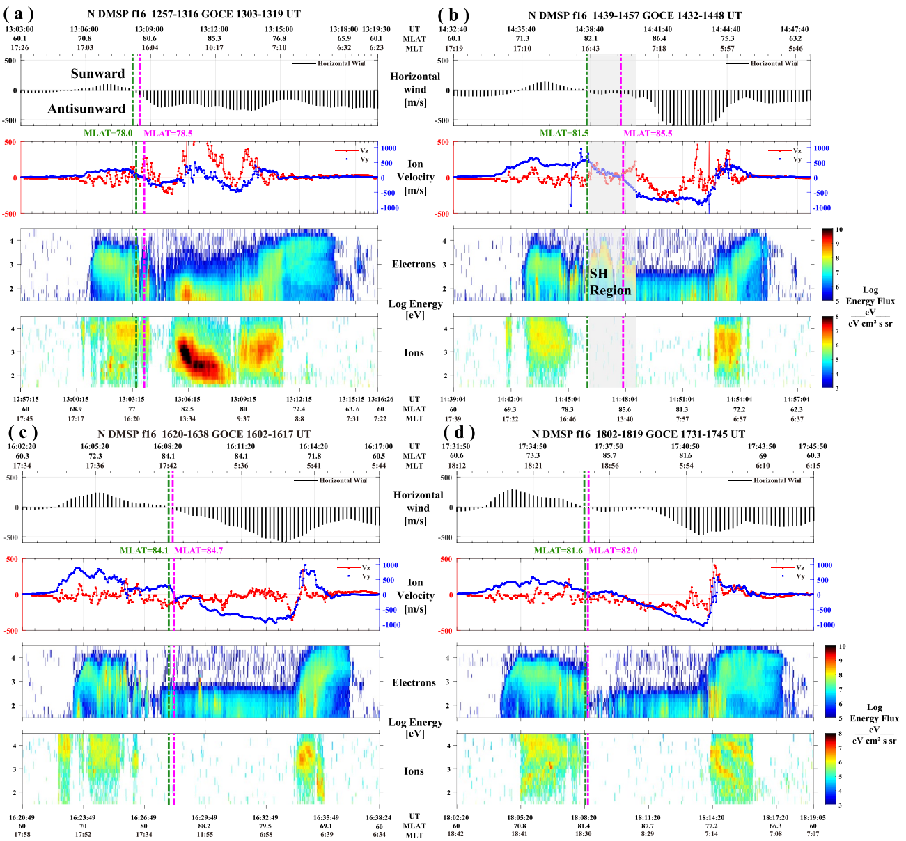
Figure 2. Each panel correspond to Figures 1c–1f. The Gravity Field and Steady-State Ocean Circulation Explorer (GOCE) orbit time and magnetic latitude is shown at the top. The Defense Meteorological Satellite Program (DMSP) orbit time, Magnetic Latitude in CGM coordinate and Magnetic Local Time in CGM coordinate is shown at the bottom. The green dotted lines represent the GOCE neutral wind reversal projected onto the DMSP measurements. The magenta dotted lines represent the DMSP V_y reversal projected onto the GOCE measurement. The space hurricane is shown as a gray shadow in panel (b). Each panel from top to bottom is: (1) GOCE horizontal wind, (2) DMSP cross-track and vertical ion velocity, (3) DMSP electron energy flux, (4) DMSP ion energy flux. The location of the ion and neutral wind reversals are indicated by magenta and green, respectively.
