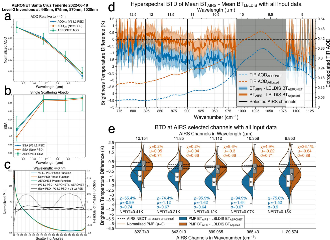
Figure 2. Dust spectral AOD normalized to 440 nm (a), SSA (b), phase functions (left y-axis in c) and residuals (gray and black curves for the right y-axis in c) at 440 nm from AERONET V3 L2 Inversions (a–c, green) and IITM calculations based on the AERONET V3 L2 PSD (a–c, blue) and the adjusted dust PSD (a–c, red). (d) The mean spectral BTDs (AIRS BT—LBLDIS BT; real curves with respect to the left y-axis from 770 to 1,130 \text{cm}^{-1} simulated using extrapolated TIR AODs (dash curves with respect to the right y-axis) based on AERONET PSD (blue) and the adjusted PSD (red), and other reference inputs indicated in Section 3.1. The gray mask represents the ozone absorption spectral regime. (e) The violin and box plots of the distribution of BTDs at the five selected AIRS channels based on AERONET PSD (blue violins, white box) and the adjusted PSD (red violins, gray box). The box boundaries and whiskers represent the 25th and 75th percentiles, and the minimum and maximum of BTDs, respectively. The \chi , \mu and \sigma represent the bias, mean and standard deviation. The brown curves represent the normalized PMF with \mu = 0 and the same \sigma as BTD distributions. The black dashed lines represent the range of AIRS NEDTs at the five channels that are listed as black texts.
