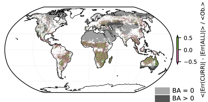
Figure 3. Mean change in out-of-sample prediction error between the CURR and ALL models, relative to mean observations ( \langle \text{Ob.} \rangle ). Green regions have decreased prediction error using the ALL model compared to the CURR model, and vice versa for the purple regions. Areas with high BA (see Fig. 2a) tend to experience lower changes in relative prediction error. Areas with very low or 0 observed BA (see Fig. 2a) are omitted to avoid division by (nearly) 0. Note that sharp data availability boundaries (e.g. in western Asia, southern Australia) are introduced by the AGB dataset. Grey shading indicates regions with fire data availability, but where one or more of the other datasets is not available. Light grey indicates regions where mean BA is 0, with dark grey representing regions with non-zero mean BA.
