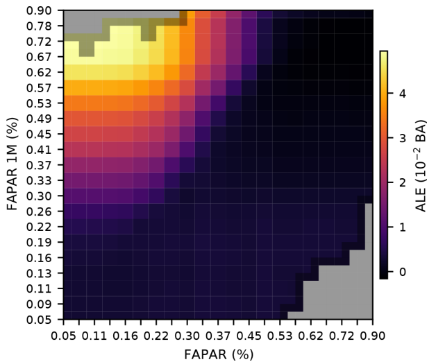
Figure 6. Second-order ALE plot showing the combined zeroth-order (mean), first-order, and second-order modelled effects of FAPAR and FAPAR 1 M on BA from the 15VEG_FAPAR model, taking into account all other variables. Grey boxes indicate missing data. See Fig. S13 for the sample count matrix which demonstrates the correlation between the variables and thus shows that samples are unlikely to fall into the top-left or bottom-right bins. Evenly spaced quantiles were used in the construction and labelling of the plots. It can be seen that the combined effect of FAPAR and FAPAR 1 M on BA is positive if FAPAR is low while FAPAR 1 M is high.
