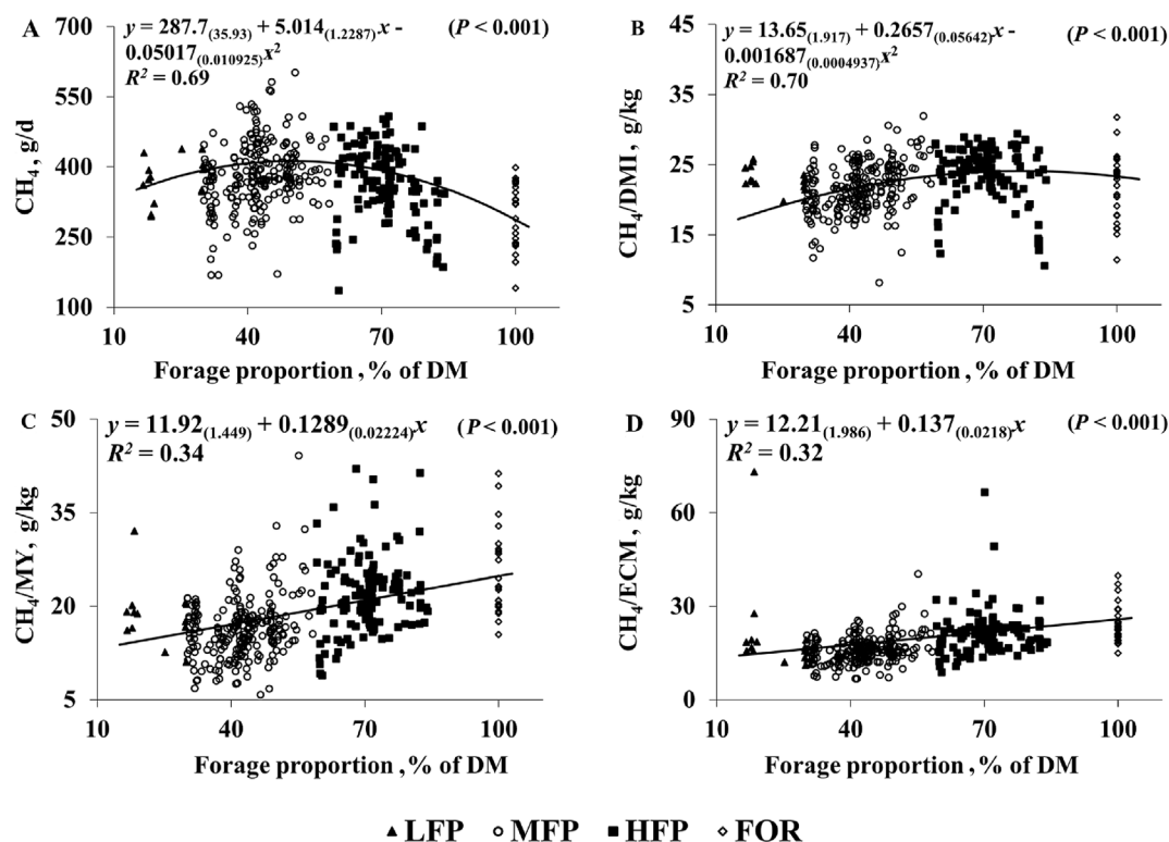
Fig. 3. Relationship between forage proportion and (A) \text{CH}_4 , (B) \text{CH}_4/\text{DMI} , (C) \text{CH}_4/\text{milk yield} , (D) \text{CH}_4/\text{ECM} for individual cows offered four experimental groups of forage proportion. LFP = 10% to 30% FP of DMI; MFP = 30% to 59% FP of DMI; HFP = 60% to 87% FP of DMI; FOR = 100% FP of DMI. \text{CH}_4 = methane; DMI = dry matter intake; DM = dry matter; MY = milk yield; ECM = energy corrected milk yield.
