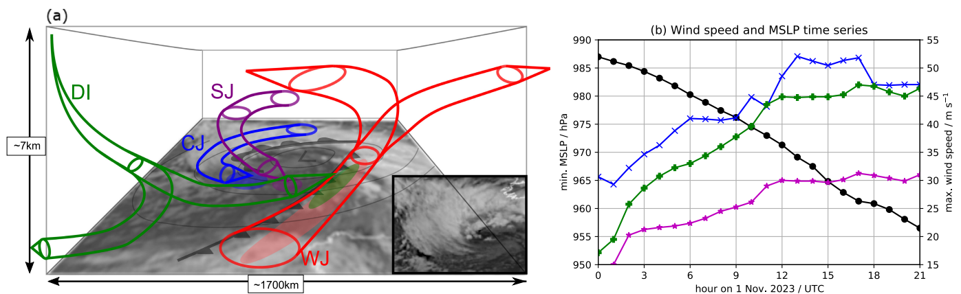
Figure 1. Evidence of possible sting jets in Storm Ciarán. (a) Schematic showing the three-dimensional airstreams that can cause strong near-surface winds in cyclones developing according to the Shapiro–Keyser conceptual model of cyclone evolution (in the Northern Hemisphere). The airstreams corresponding to the warm and cold conveyor belt jets (WJ and CJ, respectively), the sting jet (SJ) and the dry intrusion (DI) are shown by open arrows with the corresponding surface footprint indicated by an ellipse in the same colour. Mean sea-level isobars (surrounding the low-pressure centre marked by ‘L’) and surface fronts are indicated in grey by contours and conventional frontal symbols, respectively. Infrared (10.8µm) satellite imagery showing the cloud structure of Storm Ciarán as it approaches western Europe is underlain with the cloud head banding revealed in the inset cutout of the imagery which shows the cloud head tip (some editing has been applied to enhance these images). The image is a high Rate SEVIRI image from the Meteosat second-generation 0 degree satellite taken at 1700 UTC on 1 November 2023 ©EUMETSAT [2023]. (b) Time-series of maximum 850hPa windspeed (blue with crosses), 10m windspeed (magenta with stars) and 10m gusts (green with pluses) in the cold sector, and minimum MSLP (black with circles) during 1 November 2023 from the Met Office global operational forecast initialised at 0000 UTC on the same day where the cold sector is defined as where 850hPa \theta_w < 286K and within -2.5^\circ to 0.5^\circ in latitude and -5^\circ to 1^\circ in longitude of the diagnosed MSLP centre. Schematic adapted from Clark and Gray (2018) to include the DI and satellite imagery.
