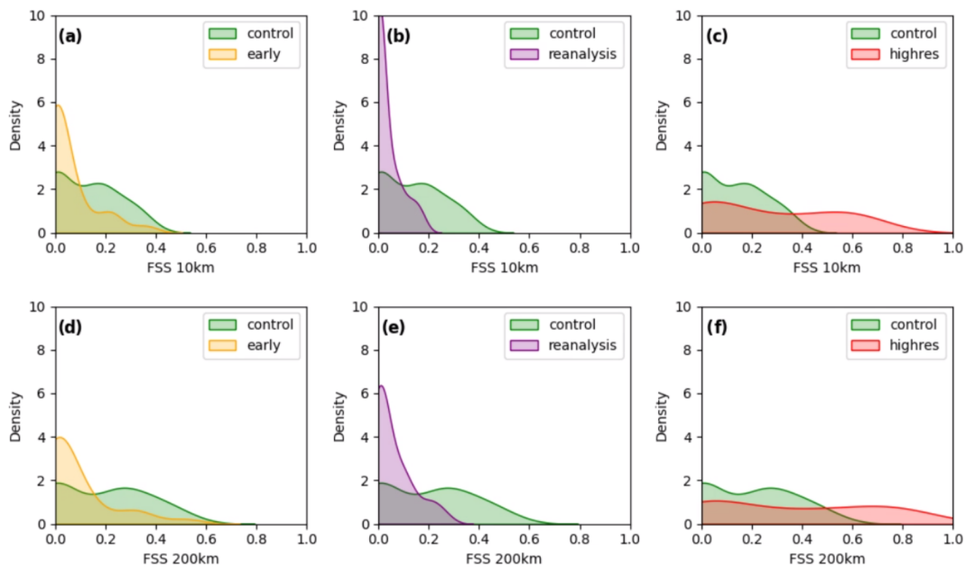
Figure 10. Fractions skill score (FSS) for the infrared 10.8 \mu\text{m} brightness temperature simulated in the control and sensitivity runs and assessed against MSG’s SEVIRI observations for a threshold of 223 K and scales of 10 km (a–c) and 200 km (d–f) for the sensitivity to initial time (a, d), initial data (b, e) and horizontal resolution (c, f). Probability distribution functions are computed over all grid points and from 18:00 UTC on 15 September to 06:00 UTC on 16 September every 3 h for the five models and variants illustrated in Fig. 9.
