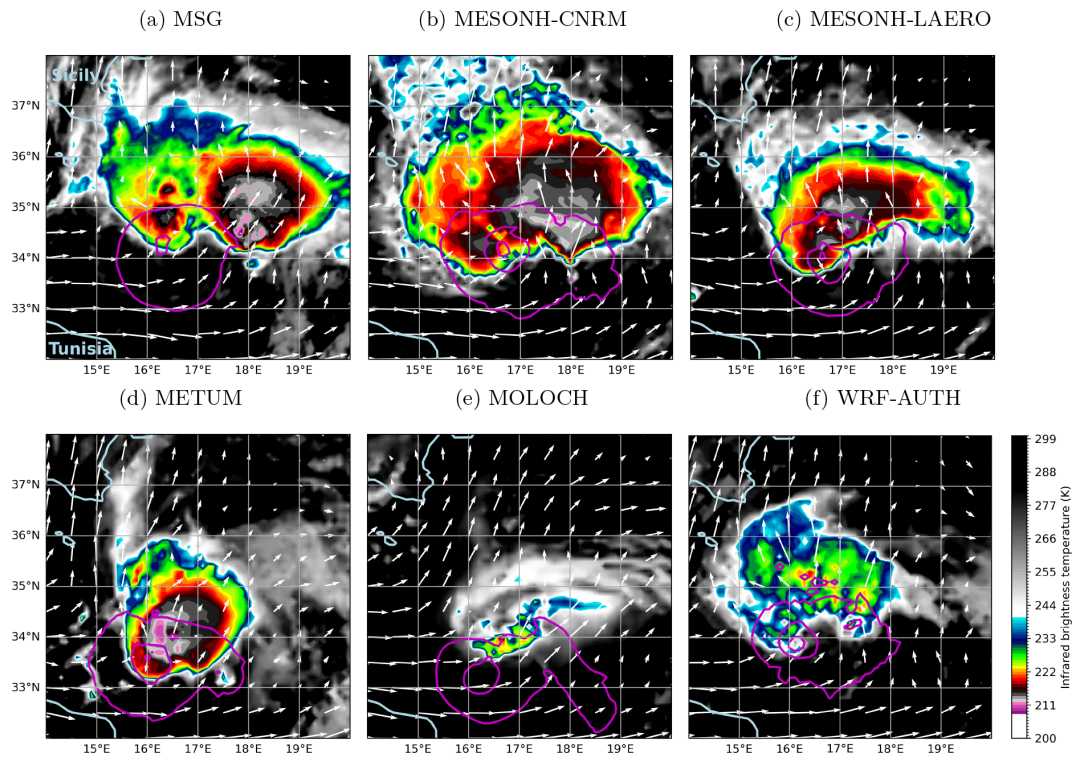
Figure 9. Infrared 10.8 \mu\text{m} brightness temperature (in K, low values highlighted) observed by Meteosat Second Generation (MSG, (a)) and simulated from high-resolution model runs (b–f) in an area of intense deep convection at 00:00 UTC on 16 September. The 300 hPa wind (vectors) and MSLP (magenta contours every 5 hPa below 1010 hPa) are overlaid from the IFS analysis in panel (a) and from the high-resolution model runs in panels (b)–(f).
