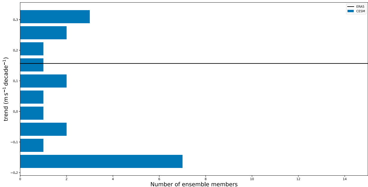
FIG. B2. Distribution of zonal wind trends in the CESM-LENS: Histogram of zonal wind speed trends at 250 hPa for the period 1980–2022 averaged between 80°–15°W and 30°–50°N for the considered CESM-LENS simulations (blue bars) and ERA5 (black line).
