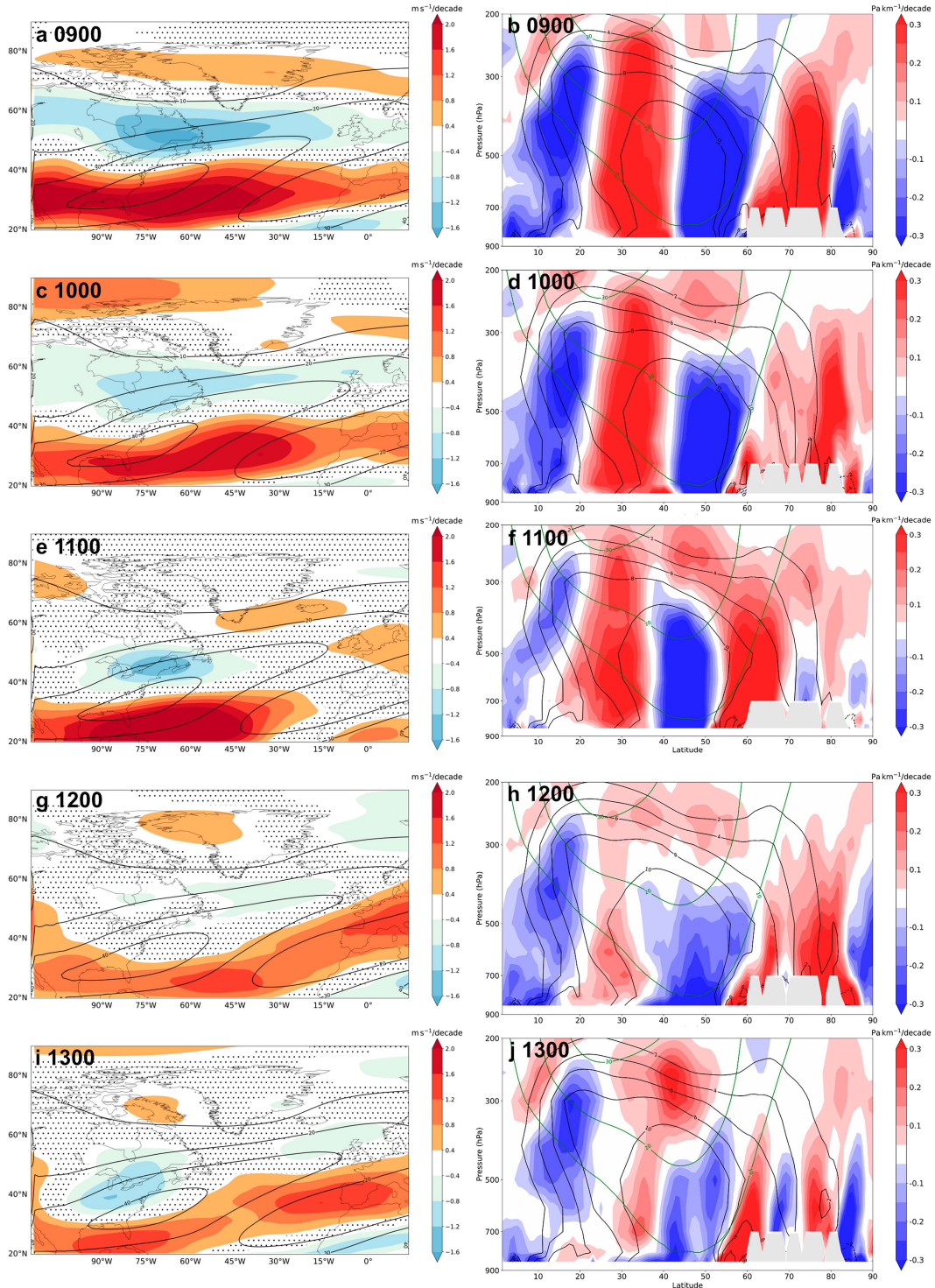
FIG. 17. Trends in 250-hPa zonal wind speed and in a vertical cross section of the slope of the isentropic surfaces for each CESM ensemble member at the end of the century period (2057–2100); as in Fig. 15, but for the end of the century period. Note the different color scales for wind trends.
