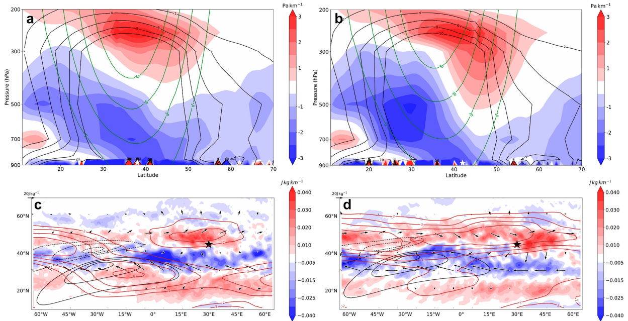
FIG. 13. Sensitivity of the baroclinicity and \mathbf{E} -vector response to the position of the SST anomaly in aquaplanet simulations: cross section of the response of the slope of the isentropic surfaces under global warming (shading) and climatological mean of slope and zonal wind in control simulations (black and green contours, respectively) with an SST anomaly located at 30°W, (a) 38°N and (b) 42°N. White stars above the x axis in (a) and (b) represent the latitudinal position of the SST anomaly. (c),(d) Response of the \mathbf{E} vector and its divergence (arrows and shading, respectively) at 250 hPa for both sensitivity experiments and response in the zonal wind at the same pressure level (brown contours). The SST anomaly is represented by black contours in (c) and (d). The stars in (c) and (d) mark a region of increased \mathbf{E} -vector divergence downstream of the SST anomaly (see text for discussion).
