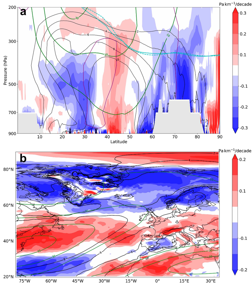
FIG. 4. DJF isentropic slope trends in ERA5 over the North Atlantic: (a) zonal mean of the trend in the slope of the isentropic surfaces between 80^{\circ} and 15^{\circ} W (shading), climatological mean slope (black contours; \text{Pa km}^{-1} ), and zonal mean zonal wind (green contours) in ERA5 (1979–2022). Blue contours represent the tropopause height (2-PVU contour) for the first (solid) and last decade (dashed) in the considered period. For reference, the contour corresponding to a potential temperature trend of 0.3 \text{ K decade}^{-1} is represented by purple lines. (b) Trend of the slope of the isentropic surfaces averaged between 250 and 850 hPa (shading), climatological mean over the same vertical layer (black contours), and climatological mean zonal wind speed at 250 hPa (green contours).
