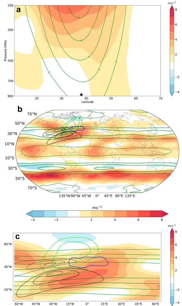
FIG. 9. Response of zonal wind speed to uniform warming in an AGCM aquaplanet simulation: (a) cross section of the zonal mean zonal wind response (shading) between 30°W and 45°E in the aquaplanet simulation with uniform warming of 4 K and the control simulation, both with an SST anomaly located at 30°W, 39°N and a climatological average of the zonal mean zonal wind over the same sector in the control simulation (green contours). The black star above the x axis indicates the latitudinal position of the SST anomaly. (b) Difference between the zonal wind speed at 250 hPa (shading), climatological mean of the zonal wind speed for the control simulation (dark green contours, between 30 and 50 \text{m s}^{-1} with dashed black contour for zero zonal wind speed), diabatic heating change (blue contour; 0.4 \text{ K day}^{-1} ), and response in the zonal 500-hPa geopotential anomalies (light green contours at -400 and -600 \text{ m}^2 \text{ s}^{-2} ). The SST anomaly is represented by black contours (from -2.5 to 2.5 \text{ K} ). To facilitate comparison with ERA5 results (Fig. 1b), all fields in (a) and (b) are shifted 50° westward. (c) Zoom of the zonal wind response, climatological zonal wind, diabatic heating, and geopotential anomalies into the area near and downstream of the SST anomaly.
