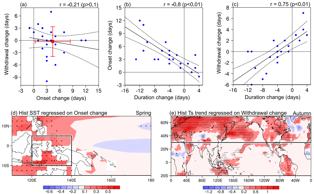
Figure 1. Inter-model relationship between future temporal shift (units: days) of the ISM: (a) onset versus withdrawal, (b) duration versus onset, and (c) duration versus withdrawal. Solid best-fit line is obtained using the least squares method, and dashed curves denote the 95% confidence range of this linear fit. The inter-model correlation coefficient ( r ) and p -value are shown on the top-right corner. The red dot (line) in (a) denotes the multi-model mean (one inter-model standard deviation). Spatial pattern of (d) historical SST ( ^{\circ}\text{C} ) in the spring (February–April) mean corresponding to future changes in ISM onset and (e) historical surface temperature trend ( ^{\circ}\text{C yr}^{-1} ) from 1960 to 2010 during autumn (September–October) corresponding to withdrawal changes, obtained by regression against the normalized future onset and withdrawal changes, respectively. The tropical mean SST between 15^{\circ}\text{S} and 15^{\circ}\text{N} in the present was removed from each model before regression. The stippling in (d), (e) represents a regression statistically significant at the 90% confidence level according to the Student's t -test. The black rectangle in (d) marks the 10^{\circ}\text{S} – 5^{\circ}\text{N} , 120^{\circ}\text{E} – 140^{\circ}\text{E} domain (WP) and in (e) denotes the 30^{\circ}\text{N} – 70^{\circ}\text{N} , 0^{\circ} – 360^{\circ}\text{E} domain (NMHL).
