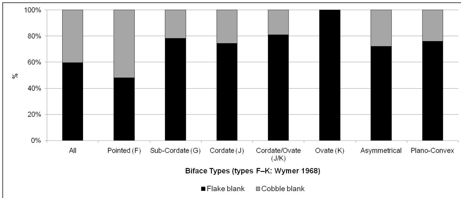
Figure 13: Proportions of blank types across the principal biface categories (types F–K after Wymer 1968) in the C.E. Bean and Exeter Museum collections
