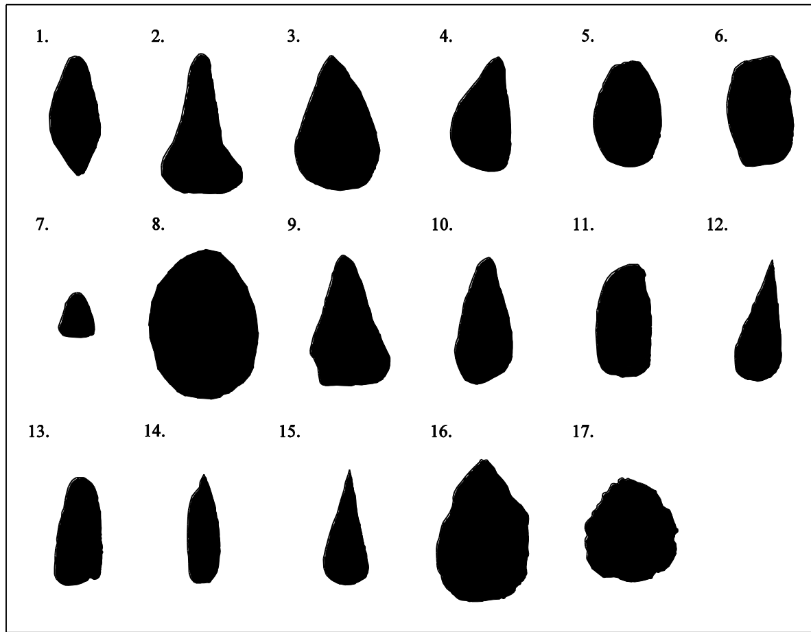
Figure 3: C.E. Bean's biface shape types (re-drawn from Bean's site notebook, held at The Dorset County Museum, Dorchester: DORCM 2005.35.AB820; ©
