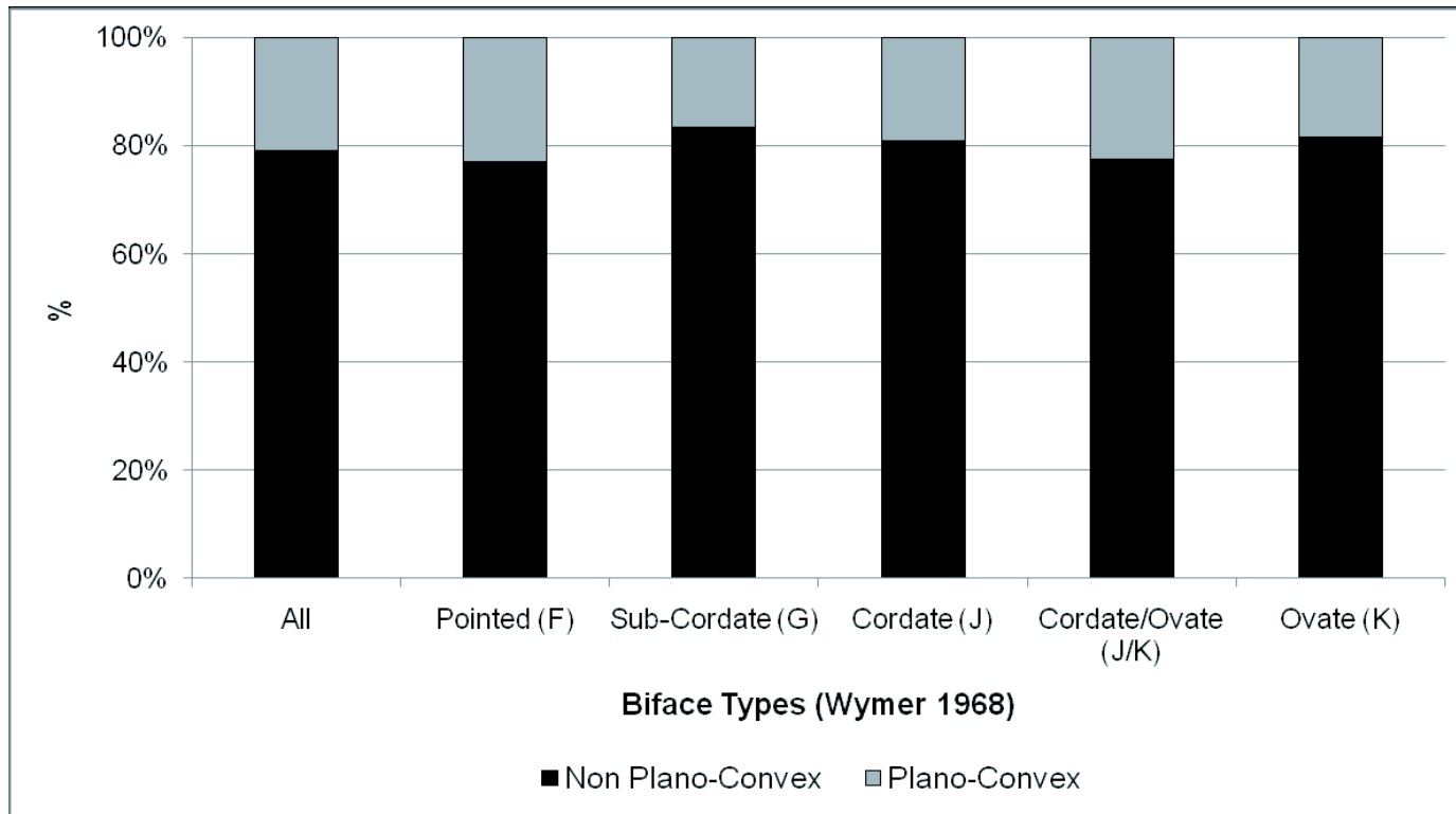
Figure 10: Proportions of plano-convex forms across the principal biface categories (after Wymer 1968) in the C.E. Bean and Exeter Museum collections
