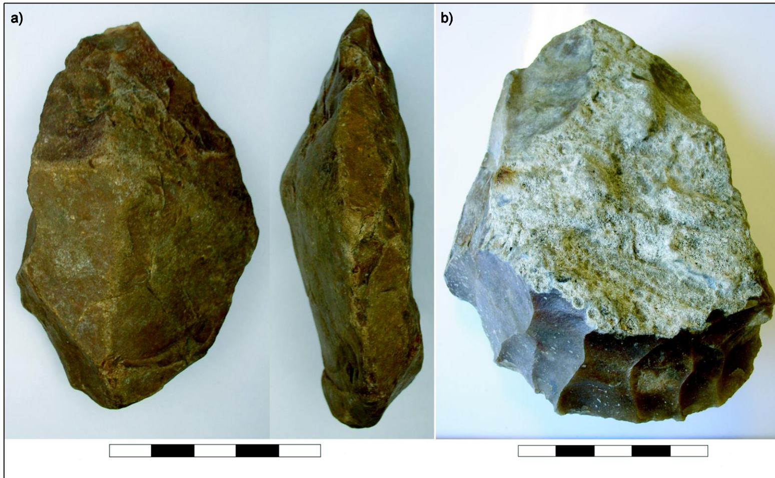
Figure 11: Chert raw materials from Broom: a) chert block collected by C.E. Bean (25.2 x 15.2 x 7.2cm); b) parallel-flaked core collected by C.E. Bean (35.6 x 22.5 x 9.8cm). 15cm scales with 3cm intervals.
