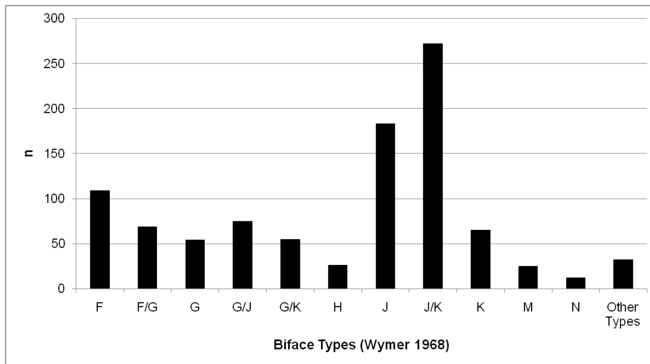
Figure 5: Biface types (after Wymer 1968) in the C.E. Bean and Exeter Museum collections. F: Pointed; F/G: Pointed/Sub-Cordate; G: Sub-Cordate; G/J: Sub-Cordate/Cordate; G/K: Sub-Cordate/Ovate; H: Cleaver; J: Cordate; J/K: Cordate/Ovate; K: Ovate; M: Ficron; N: Flat-Butted Cordate.
