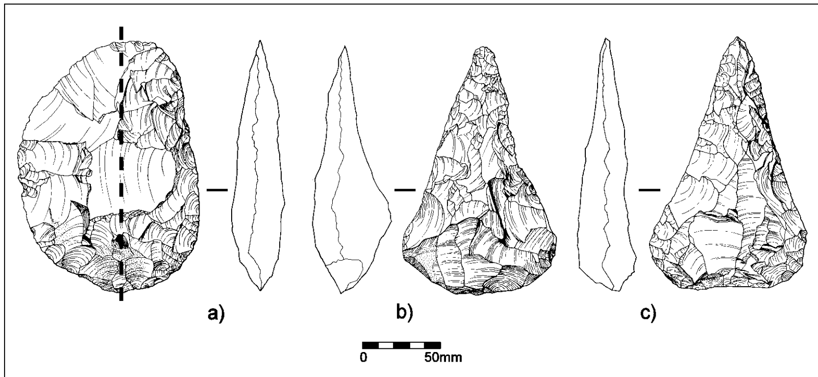
Figure 6: Examples of bifaces from Broom: a) asymmetrical forms (Bean # 1018; FlipTest (© Hardaker & Dunn) index of symmetry = 8.15 [Very low symmetry]); b) & c) points in flint (Bean # 94; FlipTest (© Hardaker & Dunn) index of symmetry = 3.15 [High symmetry]) and chert (Bean # 85; FlipTest (© Hardaker & Dunn) index of symmetry = 2.74 [Very high symmetry]) respectively. Dashed line: axis of (a)symmetry (visual classification). Illustrations by Margaret Mathews.
