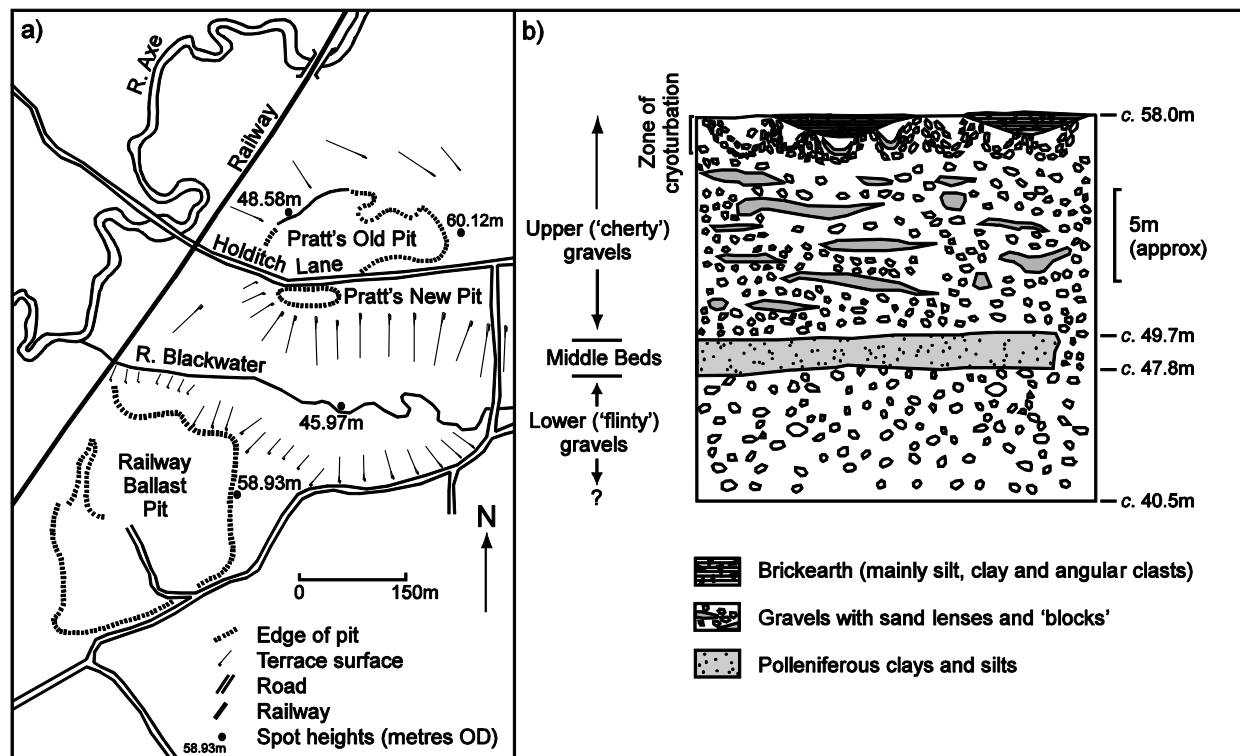
Figure 2: Gravel pit extents (a) and the geology of the Middle Pleistocene deposits (b) at Broom, Britain (after Campbell et al. 1998: Fig. 9.12, with kind permission of Springer Science and Business Media; Shakesby & Stephens 1984: Fig. 2, reproduced with the permission of the Devonshire Association). The section (b) is generalised, based on observations in all three of the Broom pits. The approximate heights are based on C.E. Bean's observations of the 'typical' stratigraphy in Pratt's Old Pit (i.e. excluding the conformable dipping of the sediments in the south-east corner of the pit: the '1938 Locality') and Dr Nick Stephens' survey in the Railway Ballast Pit.
