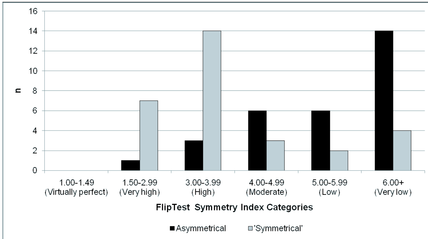
Figure 8: FlipTest (© Hardaker & Dunn) index of symmetry values for 'symmetrical' and asymmetrical bifaces in the C.E. Bean and Exeter Museum collections. Category descriptions after Hardaker & Dunn (2005).
