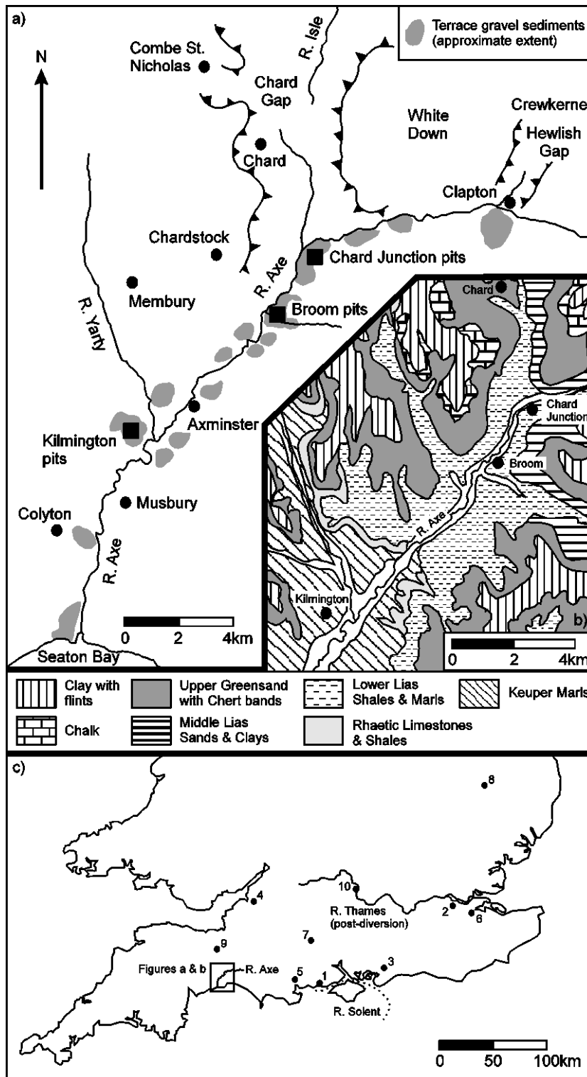
Figure 1: Location (a) and regional geology (b) of the River Axe, Britain (after Shakesby & Stephens 1984: Fig. 1) and selected British Lower Palaeolithic sites discussed in the text (c). 1a and 1b reproduced with the permission of the Devonshire Association. 1: Barton Cliff; 2: Bowman's Lodge; 3: Boxgrove; 4: Bristol Avon; 5: Corfe Mullen; 6: Cuxton; 7: Harnham; 8: Santon Downham; 9: Vale of Taunton; 10: Wallingford.
