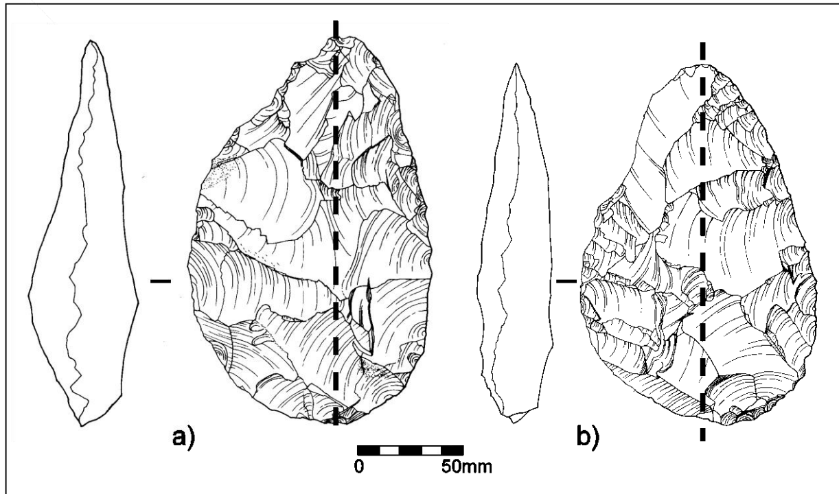
Figure 7: Examples of asymmetrical bifaces from Broom: a) Bean # 234 (FlipTest (© Hardaker & Dunn) index of symmetry = 6.66 [Very low symmetry]); b) Bean # 733 (FlipTest (© Hardaker & Dunn) index of symmetry = 4.53 [Moderate symmetry]). Dashed line: axis of (a)symmetry (visual classification).
