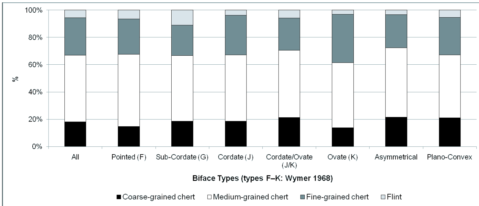
Figure 12: Proportions of raw material types across the principal biface categories (types F–K after Wymer 1968) in the C.E. Bean and Exeter Museum collections
