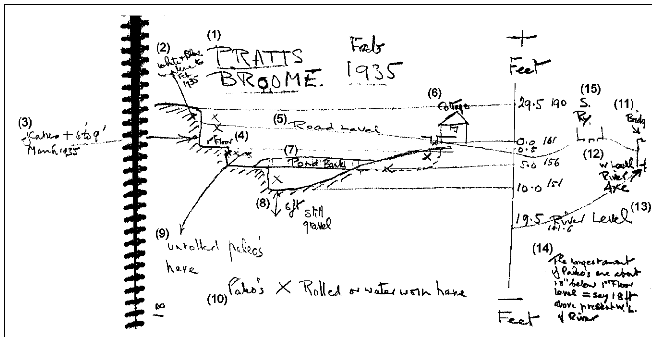
Figure 4: C.E. Bean section sketch of Pratt's Old Pit, Broom, February 1935 (modified from Bean's site notebook, held at The Dorset County Museum, Dorchester: DORCM 2005.35.AB820; © The Dorset Natural History and Archaeological Society at the Dorset County Museum). 1: Pratts Broome Feb 1935; 2: White & blue implements Feb 1935; 3: Flakes + 6' to 9' March 1935; 4: 1 st floor; 5: Road level; 6: Cottage; 7: Pond bank; 8: ↓ 6ft still gravel; 9: Unrolled palaeo's here; 10: Paleo's X Rolled or water worn here; 11: Bridge; 12: W[ater] level River Axe; 13: River level 141.6; 14: The largest amount of palaeo's are about 18" below 1 st floor level = say 18ft above present W.L. [water level] of river; 15: S[outh?] R[ailwa]y. Levels OD [feet]: 190, 161, 156, 151. Levels [feet] above/below site datum (0.0): 29.5 [above], and [all below] 0.5, 5.0, 10.0, 19.5.
