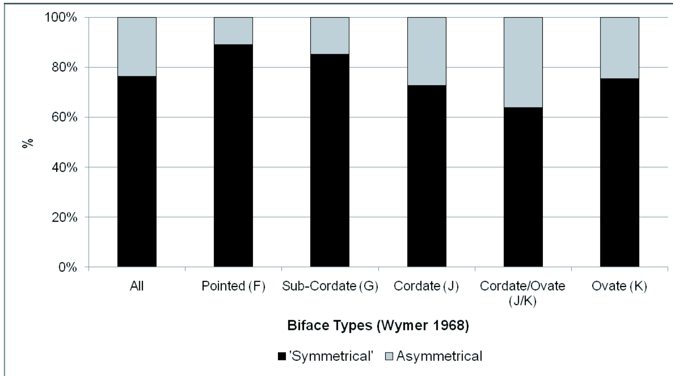
Figure 9: Proportions of asymmetrical forms across the principal biface categories (after Wymer 1968) in the C.E. Bean and Exeter Museum collections
